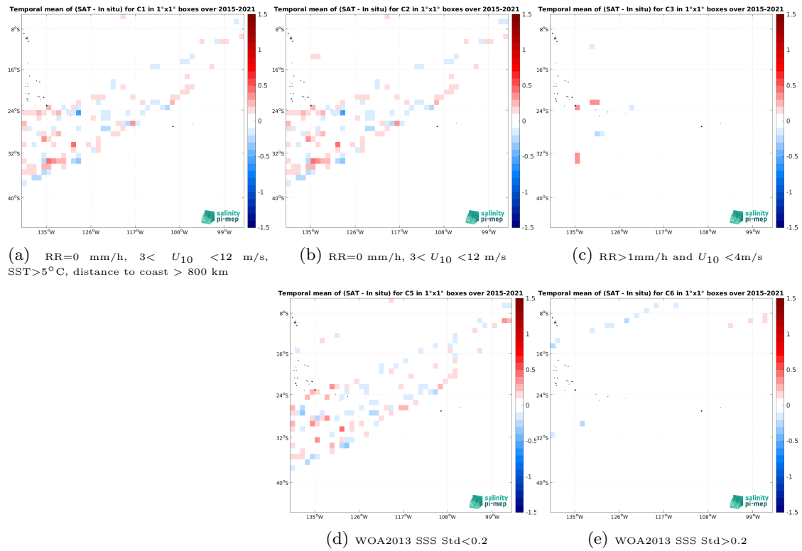
Figure 12: Temporal mean gridded over spatial boxes of size 1^\circ \times 1^\circ of \Delta SSS (SMAP SSS L3 v5 - Monthly (RSS) - TSG (LEGOS-DM)) for 5 different subdatasets corresponding to:RR=0 mm/h, 3 < U_{10} < 12 m/s, SST >5^\circ C, distance to coast > 800 km (a), RR=0 mm/h, 3 < U_{10} < 12 m/s (b), RR >1 mm/h and U_{10} < 4 m/s (c), WOA2013 SSS Std <0.2 (d), WOA2013 SSS Std >0.2 (e).
