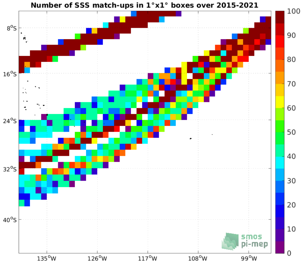
Figure 4: Number of SSS match-ups between TSG (LEGOS-DM) SSS and the SMAP SSS L3 v5 - Monthly (RSS) SSS product for the OTT zone Pi-MEP region over 1^\circ \times 1^\circ boxes and for the full satellite product period.
