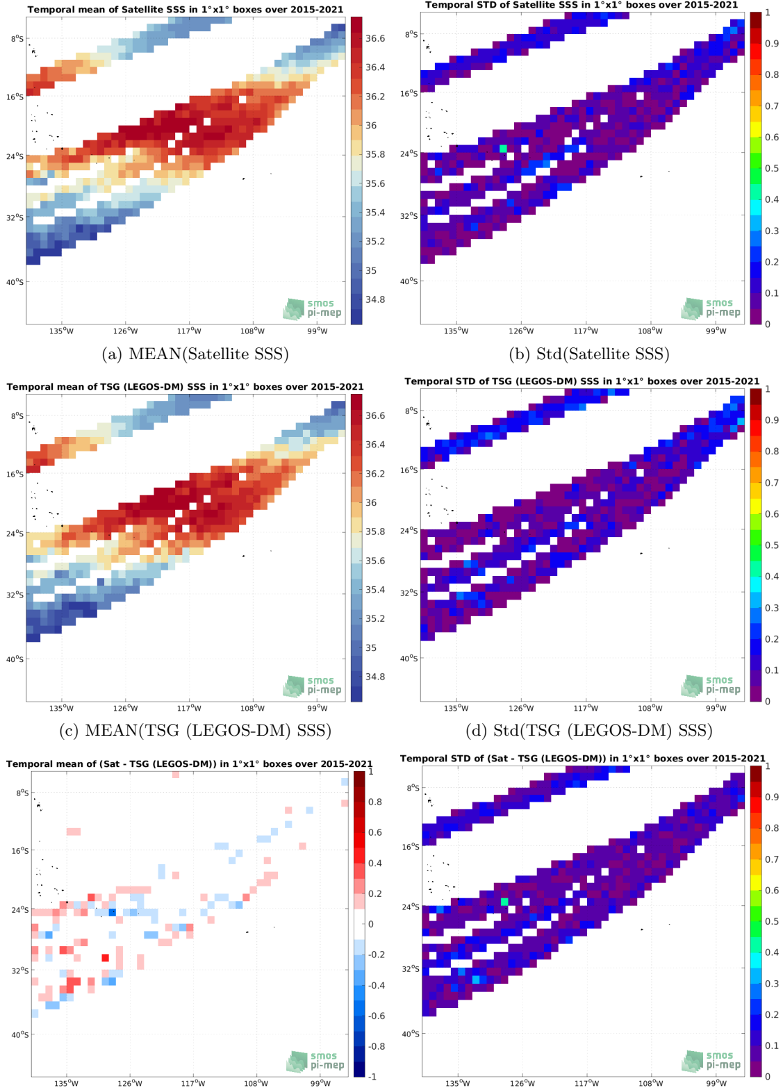
Figure 6: Temporal mean (left) and Std (right) of SSS from SMAP SSS L3 v5 - Monthly (RSS) (top), TSG (LEGOS-DM) (middle), and of \Delta SSS (Satellite - TSG (LEGOS-DM)). Only match-up pairs are used to generate these maps.
