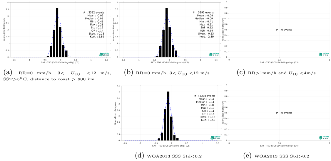
Figure 13: Normalized histogram of \Delta\text{SSS} (SMAP SSS L3 v5 - Monthly (RSS) - TSG (GOSUD-Sailing-ship)) for 5 different subdatasets corresponding to: RR=0 mm/h, 3 < U_{10} < 12 m/s, SST > 5^{\circ}\text{C} , distance to coast > 800 km (a), RR=0 mm/h, 3 < U_{10} < 12 m/s (b), RR > 1\text{mm/h} and U_{10} < 4\text{m/s} (c), WOA2013 SSS Std < 0.2 (d), WOA2013 SSS Std > 0.2 (e).
