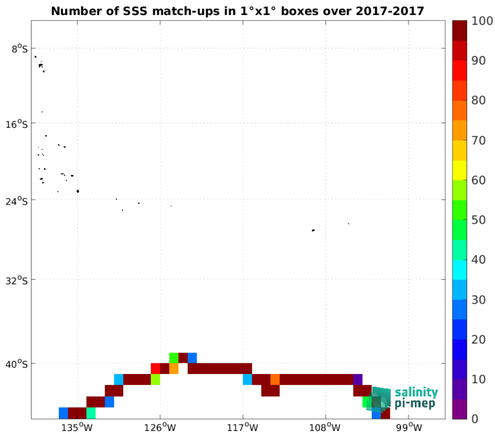
Figure 4: Number of SSS match-ups between TSG (GOSUD-Sailing-ship) SSS and the SMAP SSS L3 v5 - Monthly (RSS) SSS product for the OTT zone Pi-MEP region over 1°x1° boxes and for the full satellite product period.
