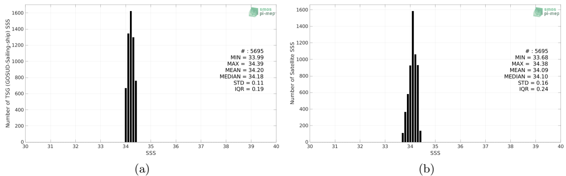
Figure 2: Histograms of SSS from TSG (GOSUD-Sailing-ship) (a) and SMAP SSS L3 v5 - Monthly (RSS) (b) considering all match-up pairs per bins of 0.1 over the OTT zone Pi-MEP region and for the full satellite product period.
