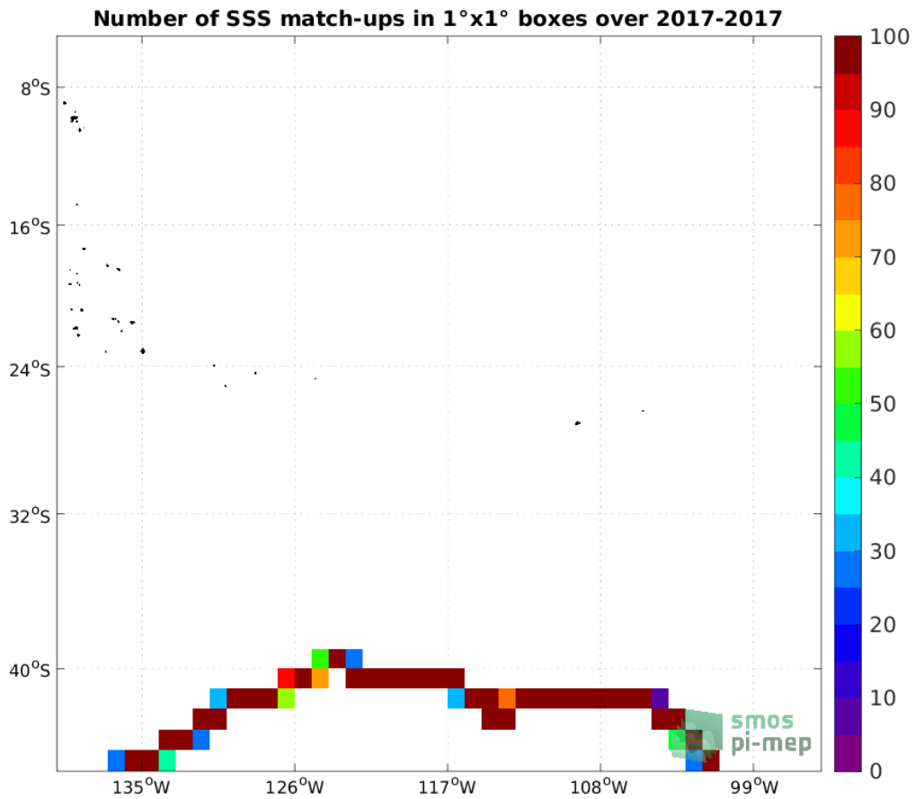
Figure 4: Number of SSS match-ups between TSG (GOSUD-Sailing-ship) SSS and the SMAP SSS L3 v5 - Monthly (RSS) SSS product for the OTT zone Pi-MEP region over 1^{\circ} \times 1^{\circ} boxes and for the full satellite product period.
