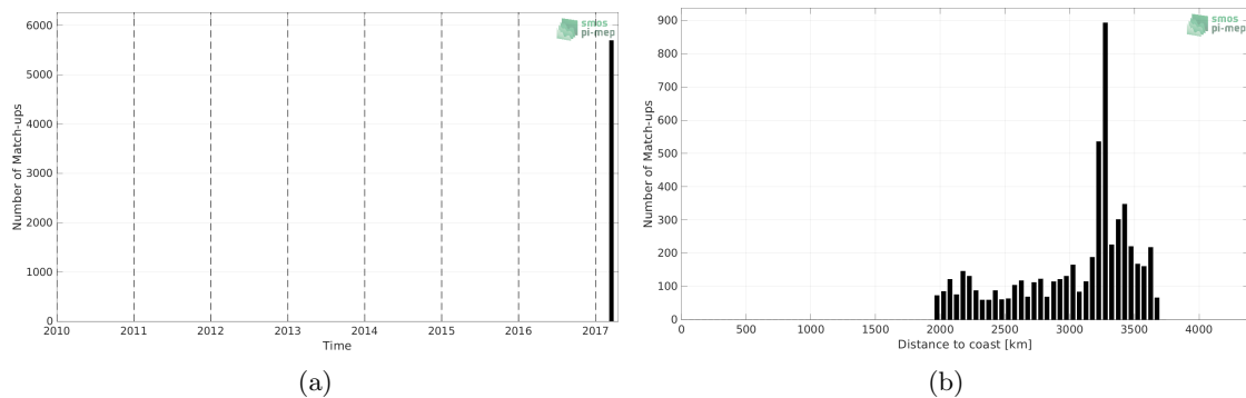
Figure 1: Number of match-ups between TSG (GOSUD-Sailing-ship) and SMAP SSS L3 v5 - Monthly (RSS) SSS as a function of time (a) and as function of the distance to coast (b) over the OTT zone Pi-MEP region and for the full satellite product period.
