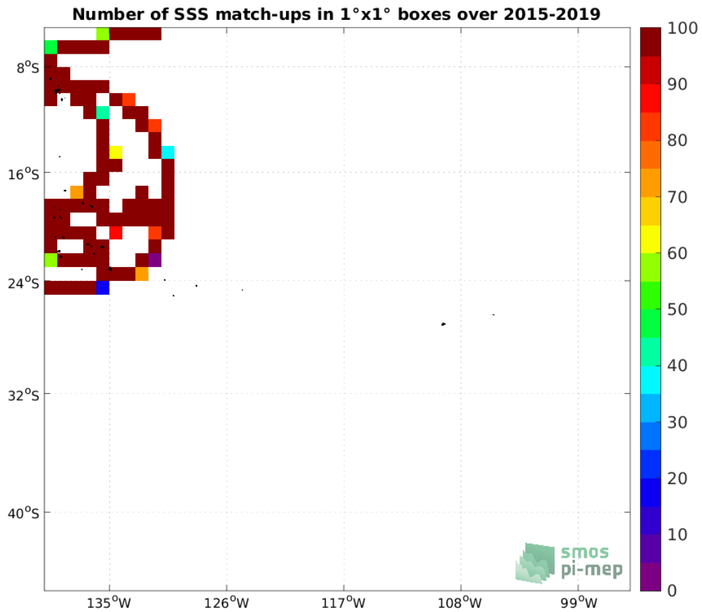
Figure 4: Number of SSS match-ups between TSG (GOSUD-Research-vessel) SSS and the SMAP SSS L3 v5 - Monthly (RSS) SSS product for the OTT zone Pi-MEP region over 1°x1° boxes and for the full satellite product period.
