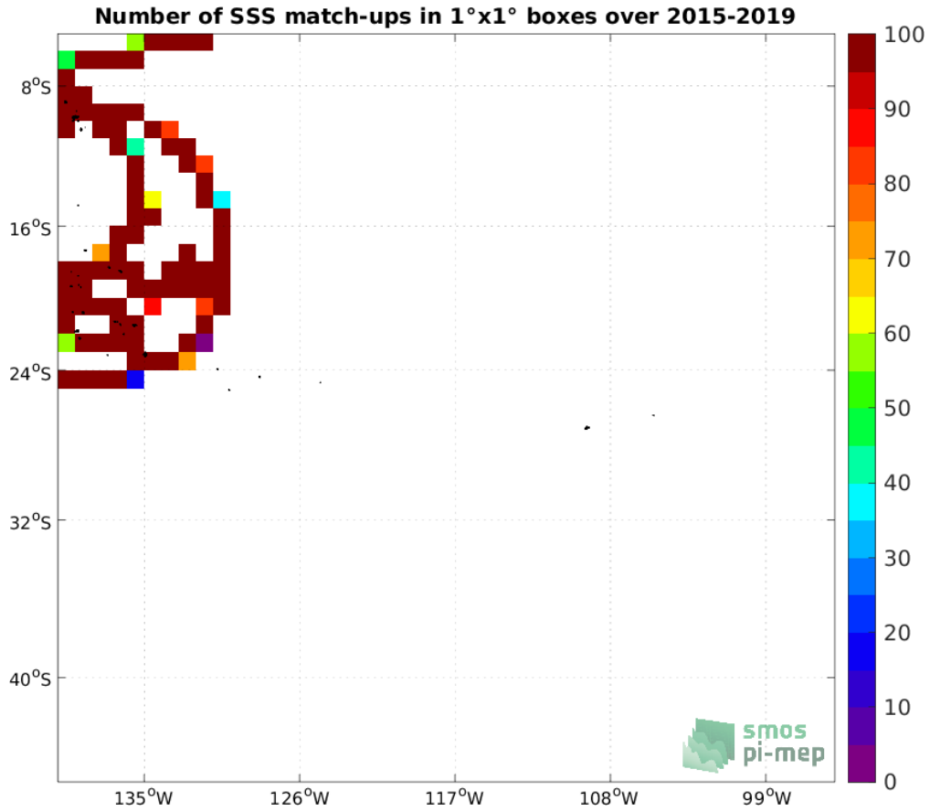
Figure 4: Number of SSS match-ups between TSG (GOSUD-Research-vessel) SSS and the SMAP SSS L3 v5 - Monthly (RSS) SSS product for the OTT zone Pi-MEP region over 1^\circ \times 1^\circ boxes and for the full satellite product period.
