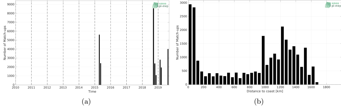
Figure 1: Number of match-ups between TSG (GOSUD-Research-vessel) and SMAP SSS L3 v5 - Monthly (RSS) SSS as a function of time (a) and as function of the distance to coast (b) over the OTT zone Pi-MEP region and for the full satellite product period.
