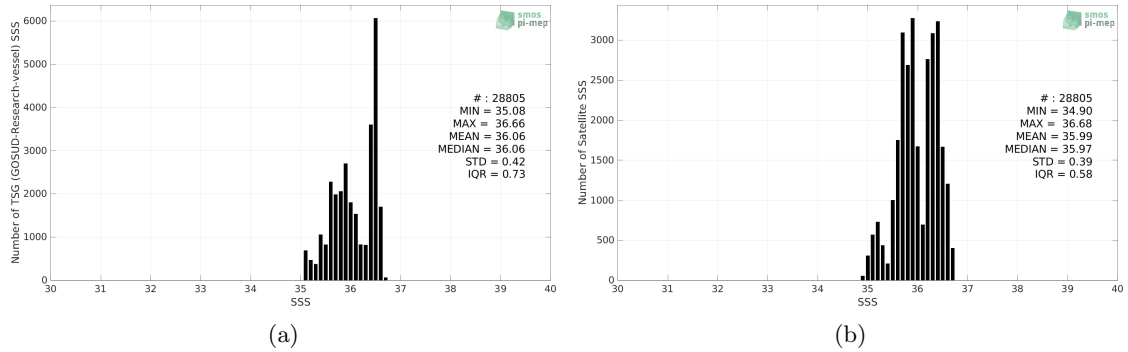
Figure 2: Histograms of SSS from TSG (GOSUD-Research-vessel) (a) and SMAP SSS L3 v5 - Monthly (RSS) (b) considering all match-up pairs per bins of 0.1 over the OTT zone Pi-MEP region and for the full satellite product period.
