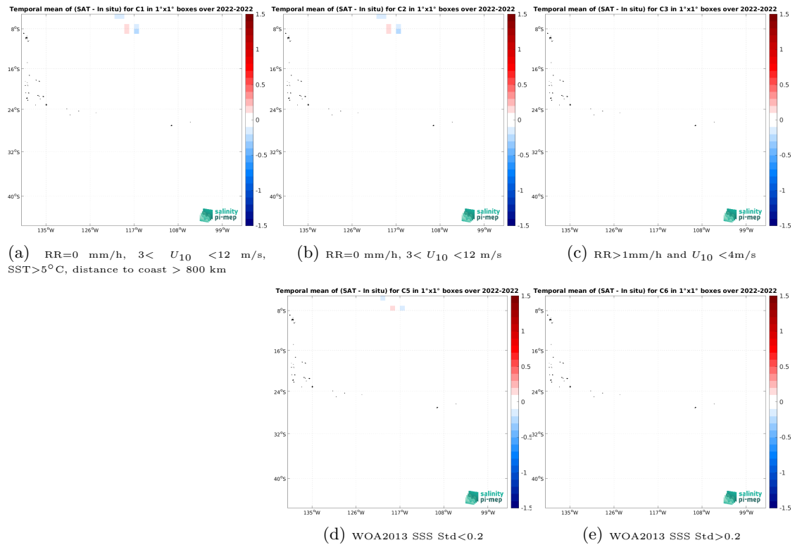
Figure 12: Temporal mean gridded over spatial boxes of size 1^\circ \times 1^\circ of \Delta SSS (SMAP SSS L3 v5 - Monthly (RSS) - Saildrone) for 5 different subdatasets corresponding to:RR=0 mm/h, 3 < U_{10} < 12 m/s, SST >5^\circ C, distance to coast > 800 km (a), RR=0 mm/h, 3 < U_{10} < 12 m/s (b), RR >1 mm/h and U_{10} < 4 m/s (c), WOA2013 SSS Std <0.2 (d), WOA2013 SSS Std >0.2 (e).
