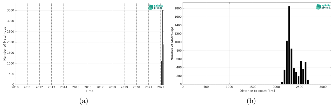
Figure 1: Number of match-ups between Saildrone and SMAP SSS L3 v5 - Monthly (RSS) SSS as a function of time (a) and as function of the distance to coast (b) over the OTT zone Pi-MEP region and for the full satellite product period.
