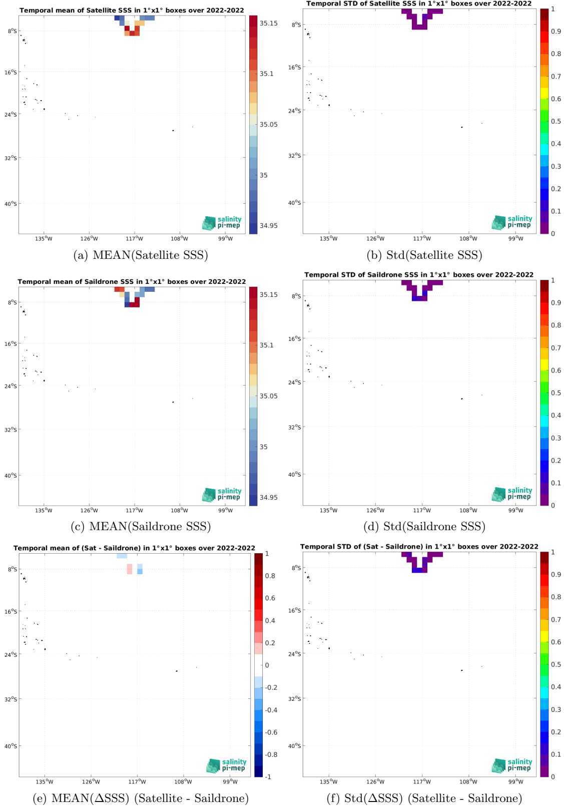
Figure 6: Temporal mean (left) and Std (right) of SSS from SMAP SSS L3 v5 - Monthly (RSS) (top), Saildrone (middle), and of \Delta SSS (Satellite - Saildrone). Only match-up pairs are used to generate these maps.
