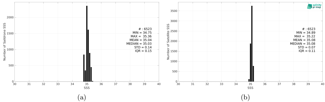
Figure 2: Histograms of SSS from Saildrone (a) and SMAP SSS L3 v5 - Monthly (RSS) (b) considering all match-up pairs per bins of 0.1 over the OTT zone Pi-MEP region and for the full satellite product period.
