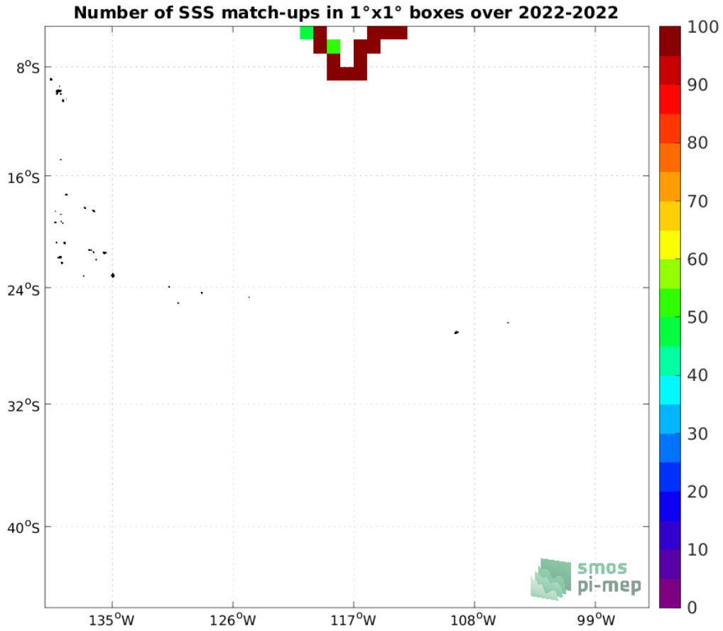
Figure 4: Number of SSS match-ups between Sairdrone SSS and the SMAP SSS L3 v5 - Monthly (RSS) SSS product for the OTT zone Pi-MEP region over 1^\circ \times 1^\circ boxes and for the full satellite product period.
