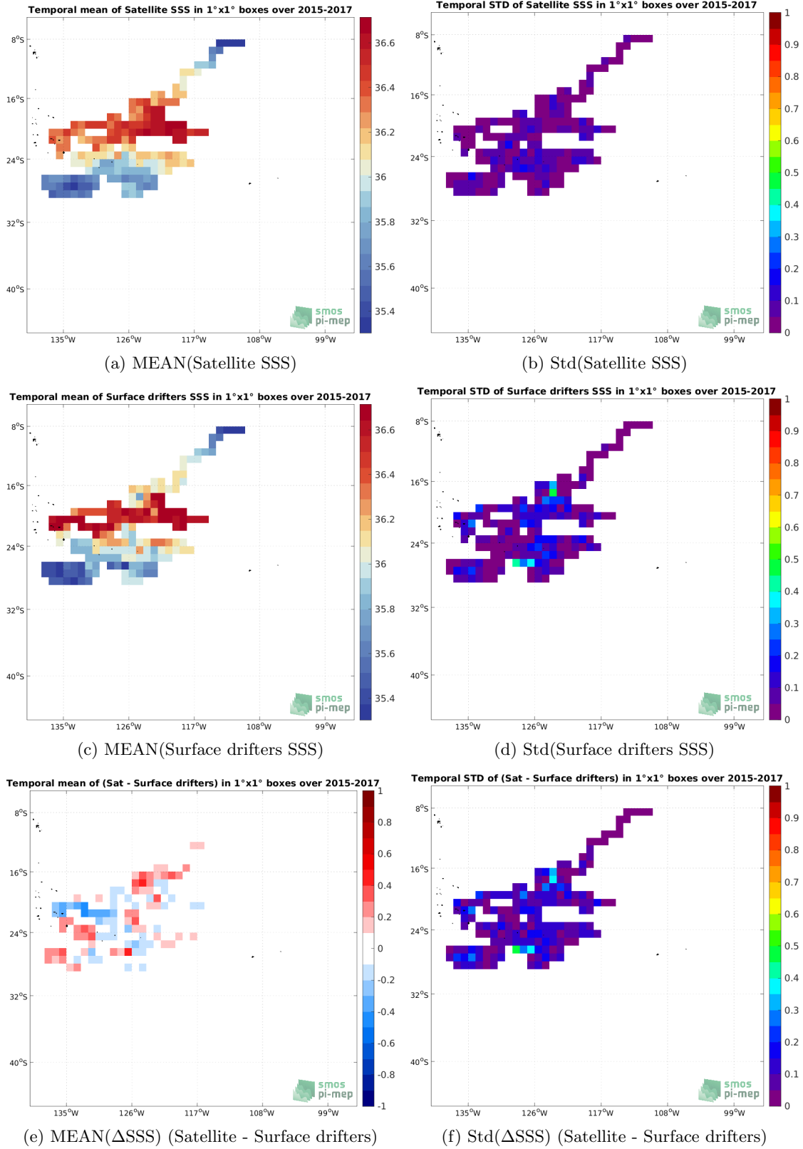
Figure 5: Temporal mean (left) and Std (right), of SSS from SMAP SSS L3 v5 - Monthly (RSS) (top), Surface drifters (middle), and of \Delta SSS (Satellite - Surface drifters). Only match-up pairs are used to generate these maps.
