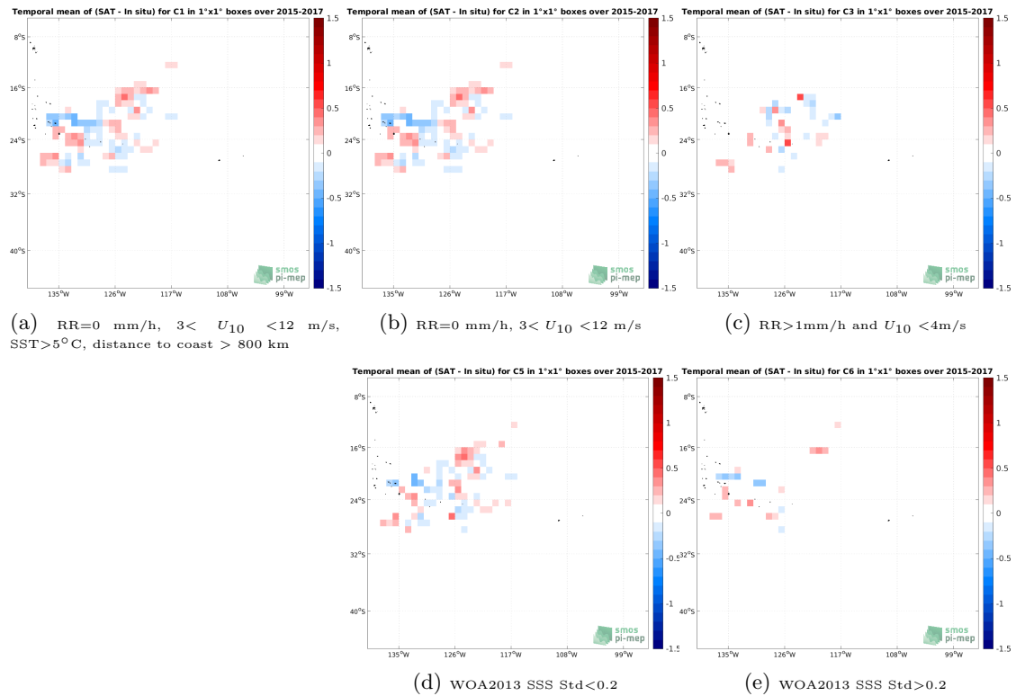
Figure 11: Temporal mean gridded over spatial boxes of size 1^\circ \times 1^\circ of \Delta SSS (SMAP SSS L3 v5 - Monthly (RSS) - Surface drifters) for 5 different subdatasets corresponding to:RR=0 mm/h, 3 < U_{10} < 12 m/s, SST >5^\circ C, distance to coast > 800 km (a), RR=0 mm/h, 3 < U_{10} < 12 m/s (b), RR >1 mm/h and U_{10} < 4 m/s (c), WOA2013 SSS Std <0.2 (d), WOA2013 SSS Std >0.2 (e).
