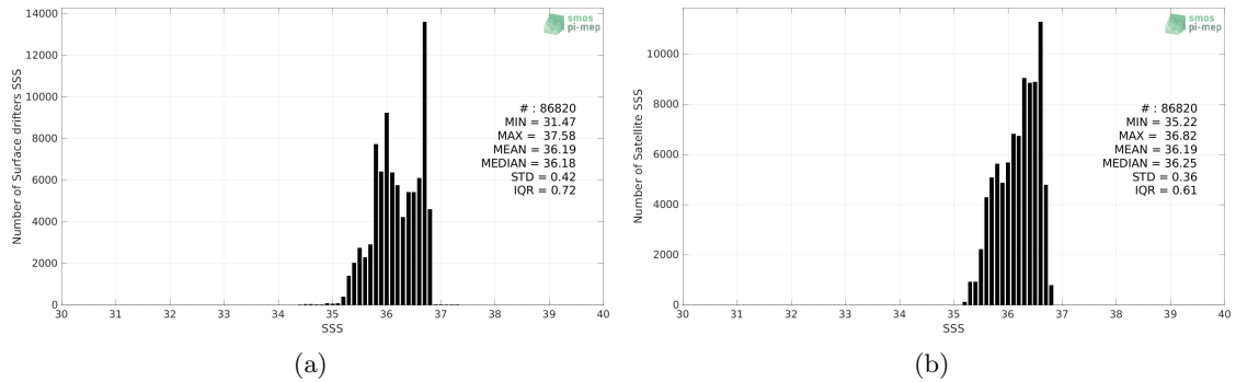
Figure 2: Histograms of SSS from Surface drifters (a) and SMAP SSS L3 v5 - Monthly (RSS) (b) considering all match-up pairs per bins of 0.1 over the OTT zone Pi-MEP region and for the full satellite product period.
