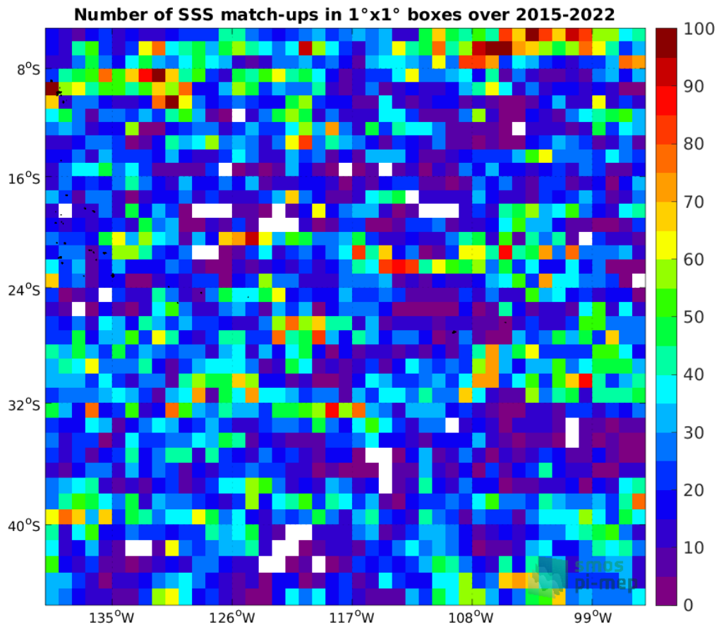
Figure 4: Number of SSS match-ups between Argo SSS and the SMAP SSS L3 v5 - Monthly (RSS) SSS product for the OTT zone Pi-MEP region over 1°x1° boxes and for the full satellite product period.
