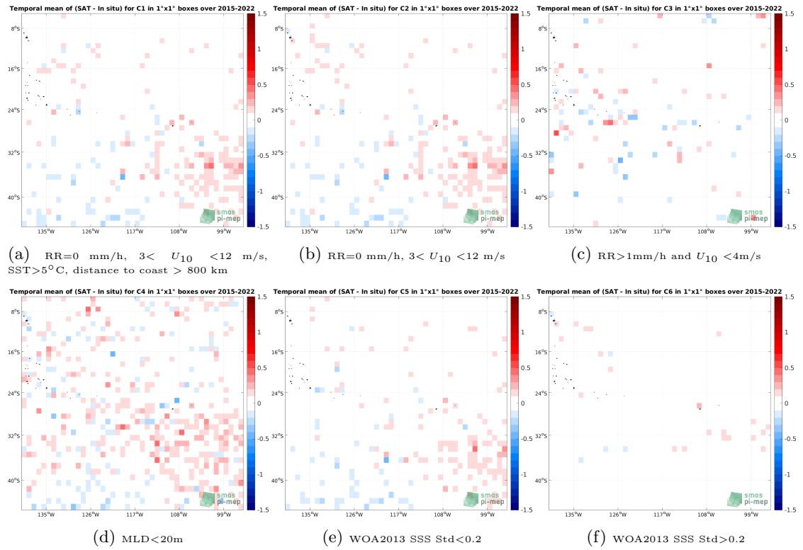
Figure 12: Temporal mean gridded over spatial boxes of size 1^\circ \times 1^\circ of \Delta SSS (SMAP SSS L3 v5 - Monthly (RSS) - Argo) for 6 different subdatasets corresponding to:RR=0 mm/h, 3 < U_{10} < 12 m/s, SST >5^\circ C, distance to coast > 800 km (a), RR=0 mm/h, 3 < U_{10} < 12 m/s (b), RR >1 mm/h and U_{10} < 4 m/s (c),MLD <20 m (d),WOA2013 SSS Std <0.2 (e),WOA2013 SSS Std >0.2 (f).
