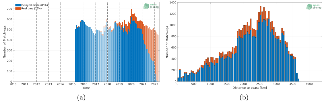
Figure 1: Number of match-ups between Argo and SMAP SSS L3 v5 - Monthly (RSS) SSS as a function of time (a) and as function of the distance to coast (b) over the OTT zone Pi-MEP region and for the full satellite product period.
