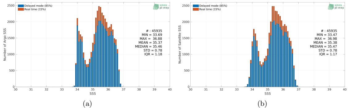
Figure 2: Histograms of SSS from Argo (a) and SMAP SSS L3 v5 - Monthly (RSS) (b) considering all match-up pairs per bins of 0.1 over the OTT zone Pi-MEP region and for the full satellite product period.
