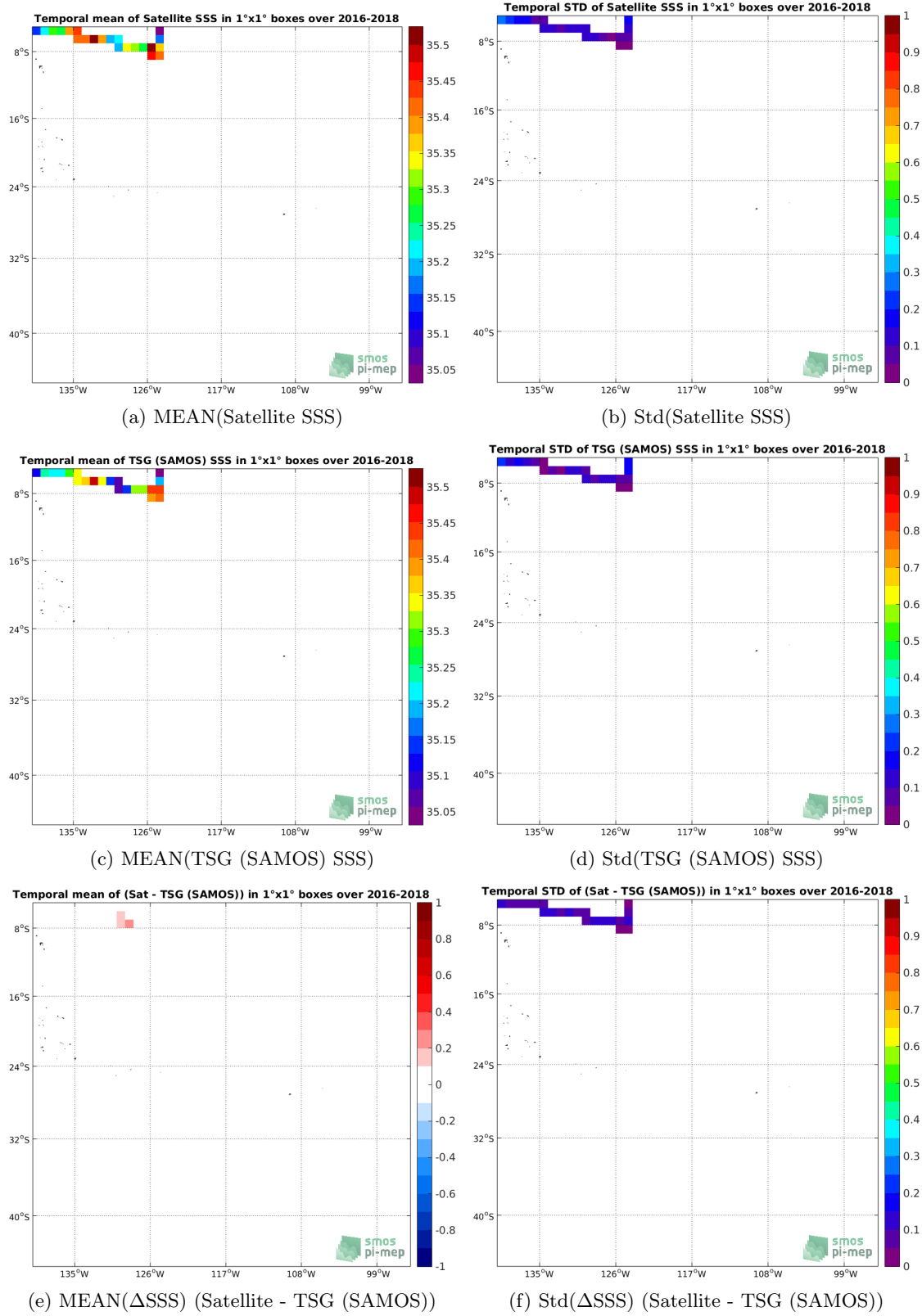
Figure 6: Temporal mean (left) and Std (right) of SSS from SMAP SSS L3 v4 - 8-Day running (RSS) (top), TSG (SAMOS) (middle), and of \Delta SSS (Satellite - TSG (SAMOS)). Only match-up pairs are used to generate these maps.
