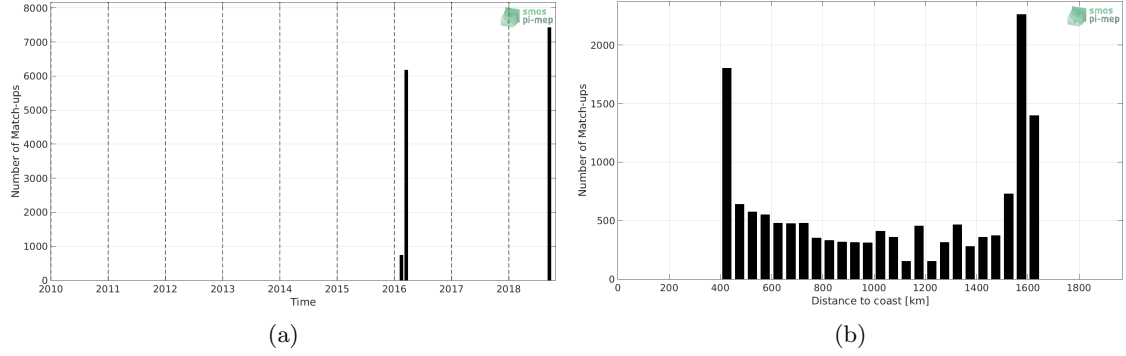
Figure 1: Number of match-ups between TSG (SAMOS) and SMAP SSS L3 v4 - 8-Day running (RSS) SSS as a function of time (a) and as function of the distance to coast (b) over the OTT zone Pi-MEP region and for the full satellite product period.
