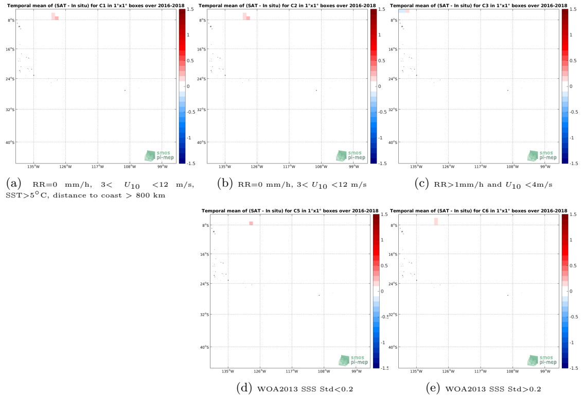
Figure 12: Temporal mean gridded over spatial boxes of size 1^\circ \times 1^\circ of \Delta SSS (SMAP SSS L3 v4 - 8-Day running (RSS) - TSG (SAMOS)) for 5 different subdatasets corresponding to: RR=0 mm/h, 3 < U_{10} < 12 m/s, SST > 5^\circ C , distance to coast > 800 km (a), RR=0 mm/h, 3 < U_{10} < 12 m/s (b), RR > 1 mm/h and U_{10} < 4 m/s (c), WOA2013 SSS Std < 0.2 (d), WOA2013 SSS Std > 0.2 (e).
