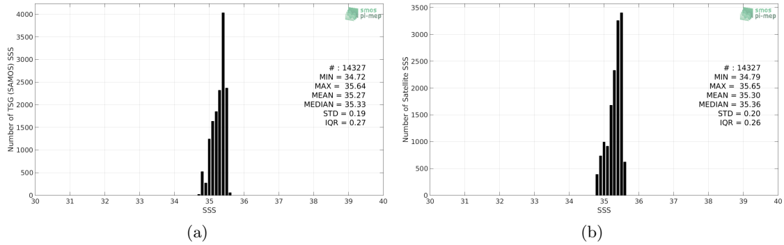
Figure 2: Histograms of SSS from TSG (SAMOS) (a) and SMAP SSS L3 v4 - 8-Day running (RSS) (b) considering all match-up pairs per bins of 0.1 over the OTT zone Pi-MEP region and for the full satellite product period.
