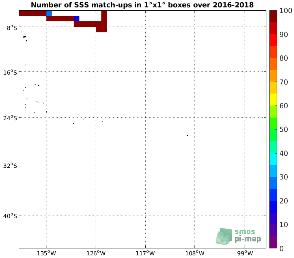
Figure 4: Number of SSS match-ups between TSG (SAMOS) SSS and the SMAP SSS L3 v4 - 8-Day running (RSS) SSS product for the OTT zone Pi-MEP region over 1°x1° boxes and for the full satellite product period.
