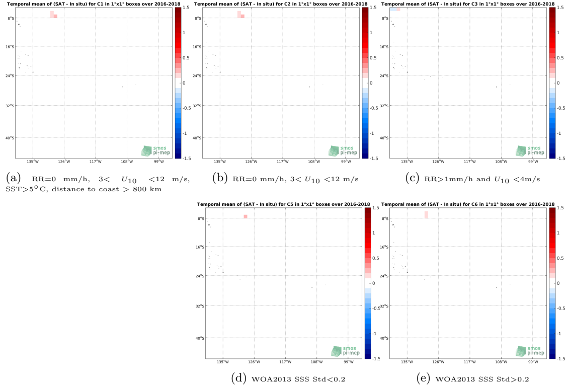
Figure 12: Temporal mean gridded over spatial boxes of size 1^\circ \times 1^\circ of \Delta SSS (SMAP-L3-RSS-V4-8DAY-RUNNING - TSG-SAMOS) for 5 different subdatasets corresponding to:RR=0 mm/h, 3 < U_{10} < 12 m/s, SST >5^\circ\text{C} , distance to coast > 800 km (a), RR=0 mm/h, 3 < U_{10} < 12 m/s (b), RR >1 mm/h and U_{10} < 4 m/s (c), WOA2013 SSS Std <0.2 (d), WOA2013 SSS Std >0.2 (e).
