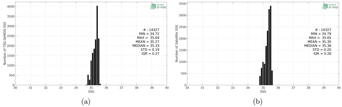
Figure 2: Histograms of SSS from TSG-SAMOS (a) and SMAP-L3-RSS-V4-8DAY-RUNNING (b) considering all match-up pairs per bins of 0.1 over the OTT zone Pi-MEP region and for the full satellite product period.
