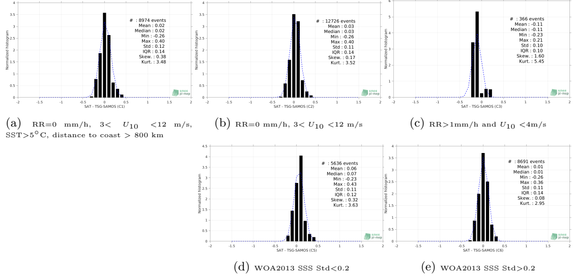
Figure 13: Normalized histogram of \Delta\text{SSS} (SMAP-L3-RSS-V4-8DAY-RUNNING - TSG-SAMOS) for 5 different subdatasets corresponding to: RR=0 mm/h, 3 < U_{10} < 12 m/s, SST > 5^{\circ}\text{C} , distance to coast > 800 km (a), RR=0 mm/h, 3 < U_{10} < 12 m/s (b), RR > 1\text{mm/h} and U_{10} < 4\text{m/s} (c), WOA2013 SSS \text{Std} < 0.2 (d), WOA2013 SSS \text{Std} > 0.2 (e).
