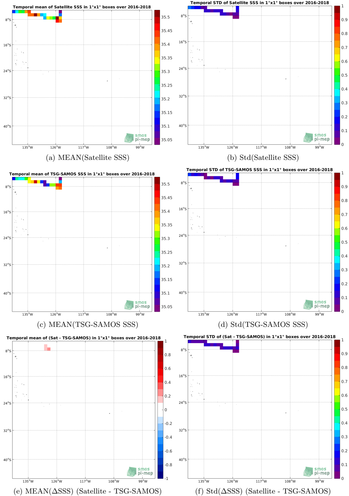
Figure 6: Temporal mean (left) and Std (right) of SSS from SMAP-L3-RSS-V4-8DAY-RUNNING (top), TSG-SAMOS (middle), and of \Delta SSS (Satellite - TSG-SAMOS). Only match-up pairs are used to generate these maps.
