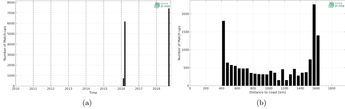
Figure 1: Number of match-ups between TSG-SAMOS and SMAP-L3-RSS-V4-8DAY-RUNNING SSS as a function of time (a) and as function of the distance to coast (b) over the OTT zone Pi-MEP region and for the full satellite product period.
