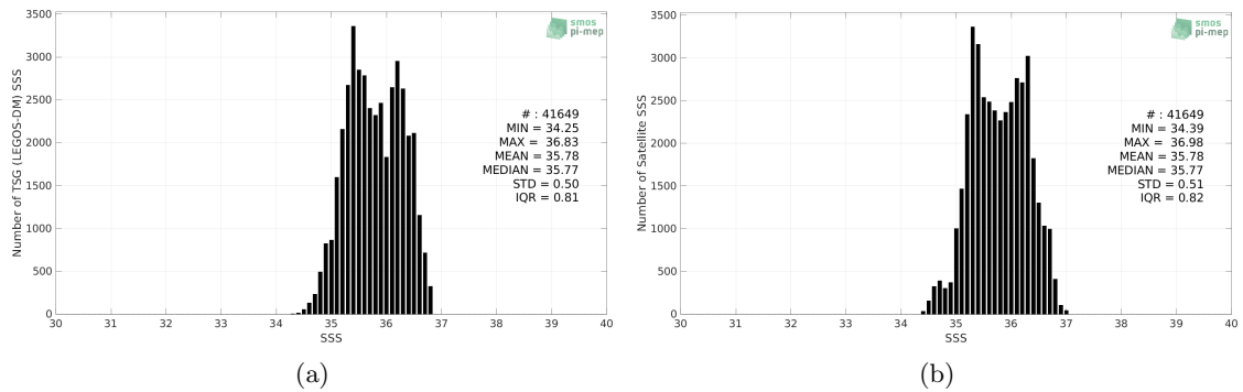
Figure 2: Histograms of SSS from TSG (LEGOS-DM) (a) and SMAP SSS L3 v4 - 8-Day running (RSS) (b) considering all match-up pairs per bins of 0.1 over the OTT zone Pi-MEP region and for the full satellite product period.
