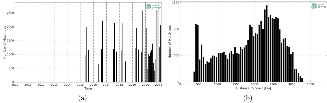
Figure 1: Number of match-ups between TSG (LEGOS-DM) and SMAP SSS L3 v4 - 8-Day running (RSS) SSS as a function of time (a) and as function of the distance to coast (b) over the OTT zone Pi-MEP region and for the full satellite product period.
