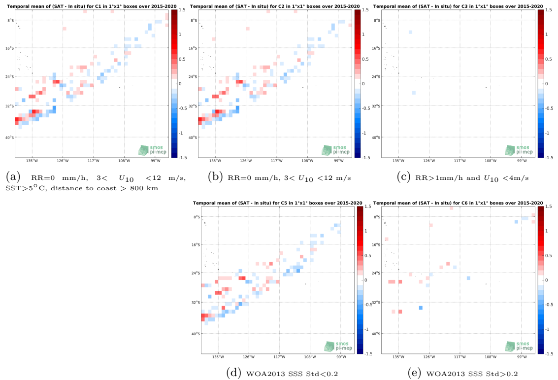
Figure 12: Temporal mean gridded over spatial boxes of size 1^\circ \times 1^\circ of \Delta\text{SSS} (SMAP SSS L3 v4 - 8-Day running (RSS) - TSG (LEGOS-DM)) for 5 different subdatasets corresponding to:RR=0 mm/h, 3 < U_{10} < 12 m/s, SST >5^\circ\text{C} , distance to coast > 800 km (a), RR=0 mm/h, 3 < U_{10} < 12 m/s (b), RR >1 mm/h and U_{10} < 4 m/s (c), WOA2013 SSS Std <0.2 (d), WOA2013 SSS Std >0.2 (e).
