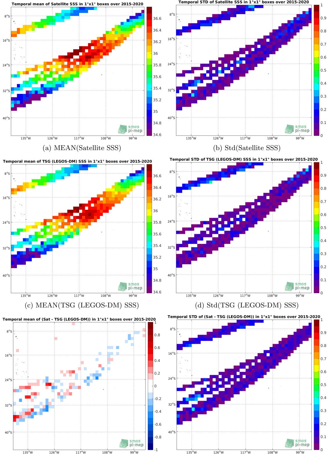
Figure 6: Temporal mean (left) and Std (right) of SSS from SMAP SSS L3 v4 - 8-Day running (RSS) (top), TSG (LEGOS-DM) (middle), and of \Delta SSS (Satellite - TSG (LEGOS-DM)). Only match-up pairs are used to generate these maps.
