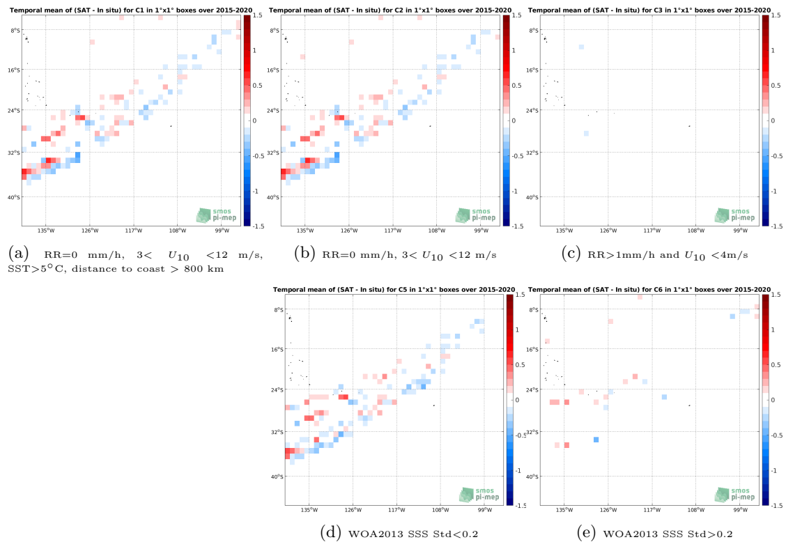
Figure 12: Temporal mean gridded over spatial boxes of size 1^\circ \times 1^\circ of \Delta\text{SSS} (SMAP SSS L3 v4 - 8-Day running (RSS) - TSG (LEGOS-DM)) for 5 different subdatasets corresponding to:RR=0 mm/h, 3 < U_{10} < 12 m/s, SST >5^\circ\text{C} , distance to coast > 800 km (a), RR=0 mm/h, 3 < U_{10} < 12 m/s (b), RR >1 mm/h and U_{10} < 4 m/s (c), WOA2013 SSS Std <0.2 (d), WOA2013 SSS Std >0.2 (e).
