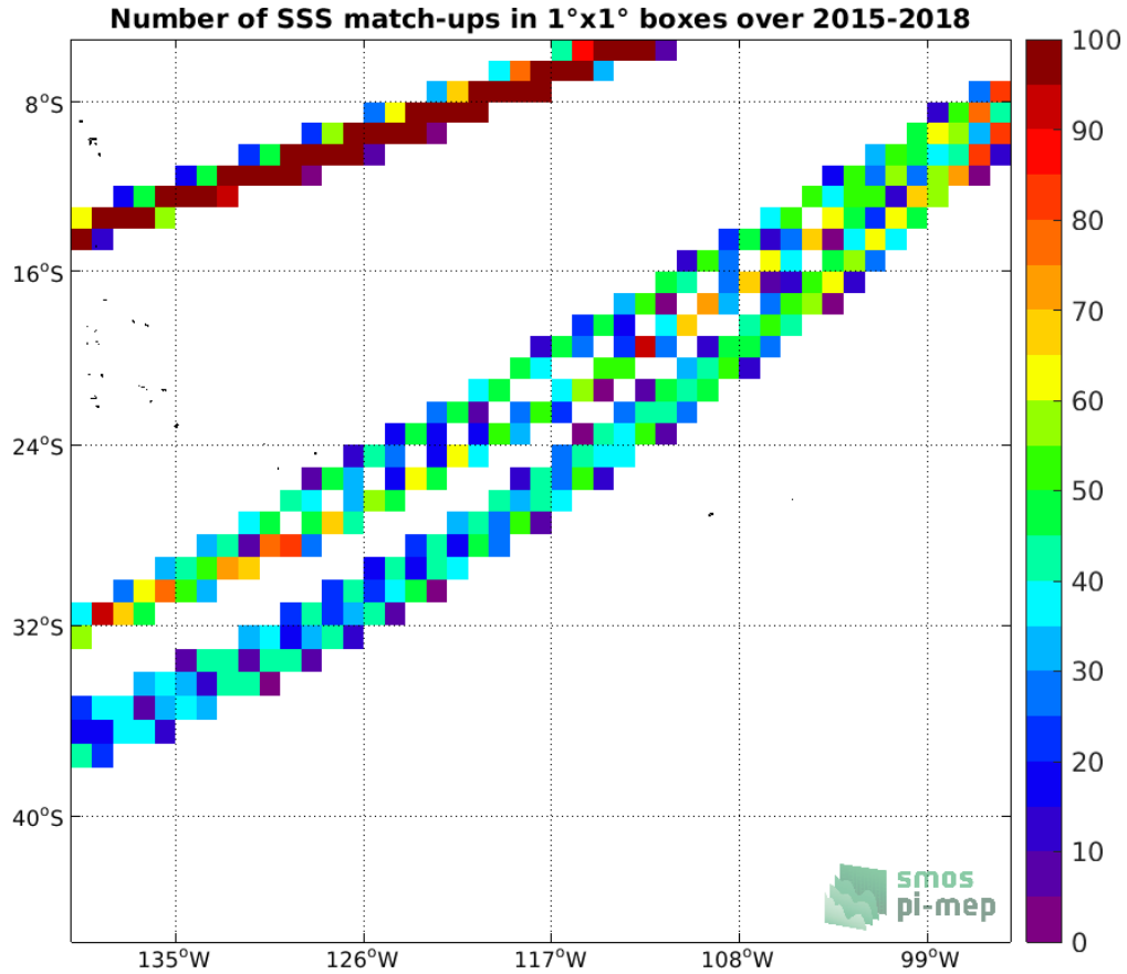
Figure 4: Number of SSS match-ups between TSG (LEGOS-DM) SSS and the SMAP SSS L3 v4 - 8-Day running (RSS) SSS product for the OTT zone Pi-MEP region over 1°x1° boxes and for the full satellite product period.
