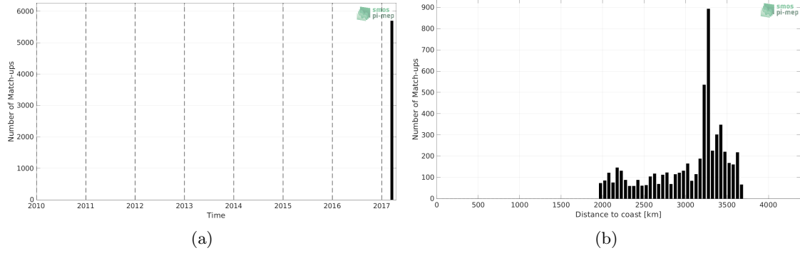
Figure 1: Number of match-ups between TSG (GOSUD-Sailing-ship) and SMAP SSS L3 v4 - 8-Day running (RSS) SSS as a function of time (a) and as function of the distance to coast (b) over the OTT zone Pi-MEP region and for the full satellite product period.
