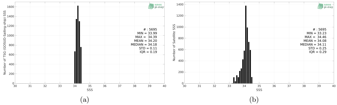
Figure 2: Histograms of SSS from TSG (GOSUD-Sailing-ship) (a) and SMAP SSS L3 v4 - 8-Day running (RSS) (b) considering all match-up pairs per bins of 0.1 over the OTT zone Pi-MEP region and for the full satellite product period.
