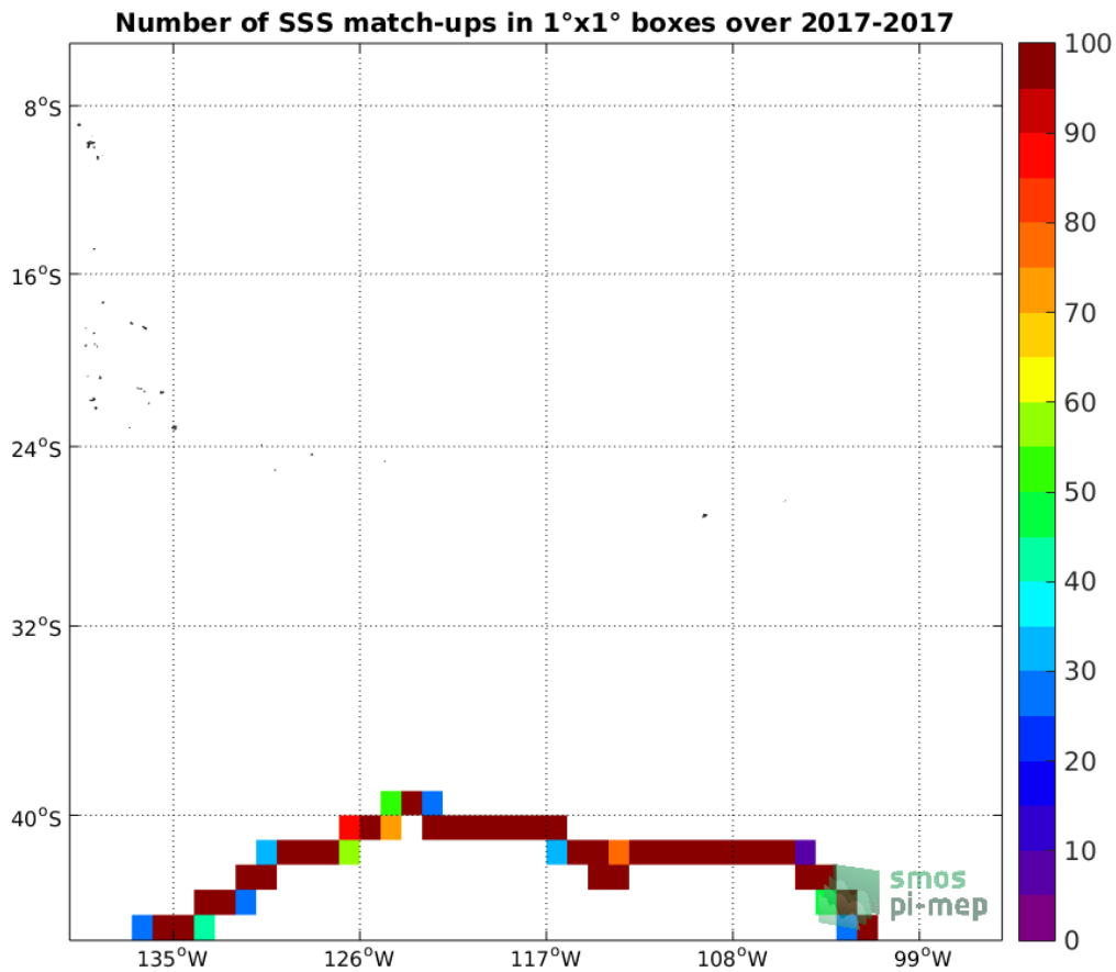
Figure 4: Number of SSS match-ups between TSG (GOSUD-Sailing-ship) SSS and the SMAP SSS L3 v4 - 8-Day running (RSS) SSS product for the OTT zone Pi-MEP region over 1°x1° boxes and for the full satellite product period.
