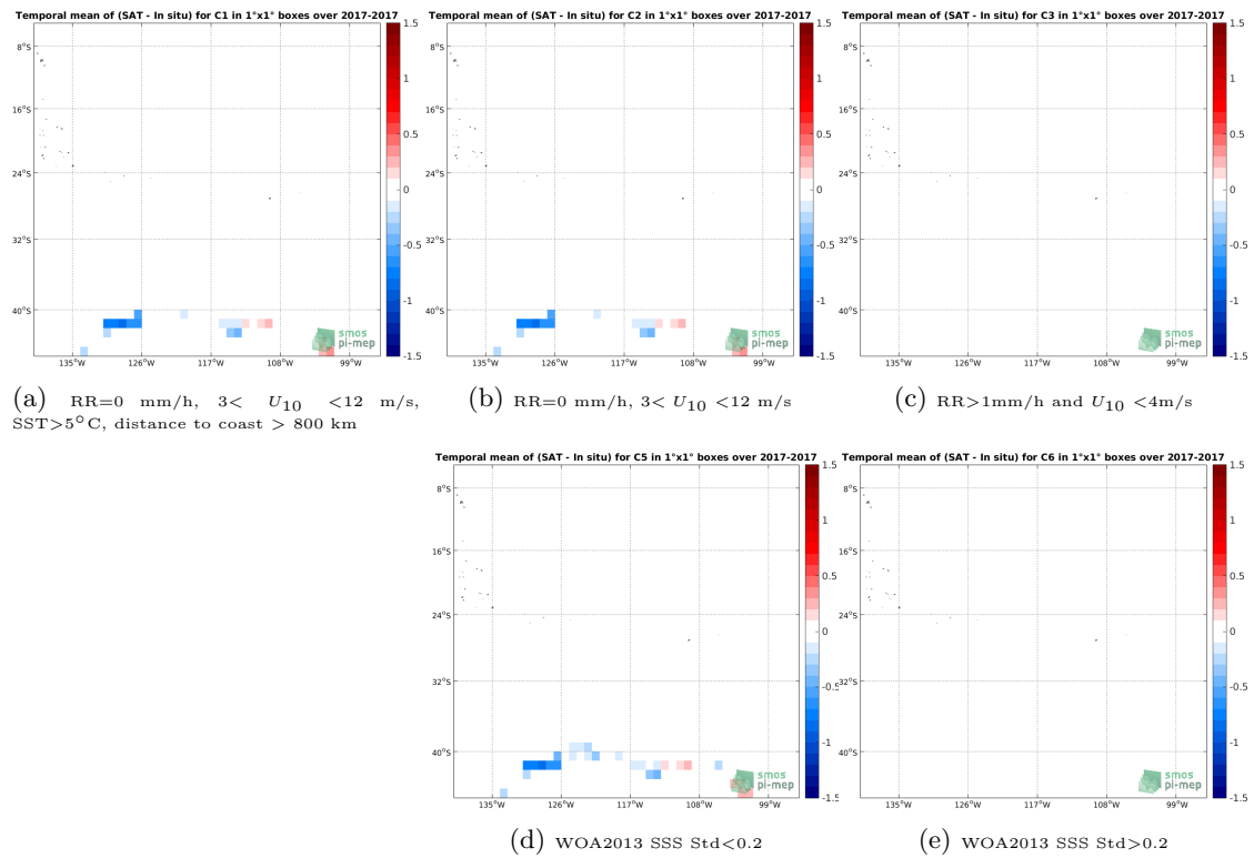
Figure 12: Temporal mean gridded over spatial boxes of size 1^\circ \times 1^\circ of \Delta\text{SSS} (SMAP SSS L3 v4 - 8-Day running (RSS) - TSG (GOSUD-Sailing-ship)) for 5 different subdatasets corresponding to: RR=0 mm/h, 3 < U_{10} < 12 m/s, SST > 5°C, distance to coast > 800 km (a), RR=0 mm/h, 3 < U_{10} < 12 m/s (b), RR > 1mm/h and U_{10} < 4 m/s (c), WOA2013 SSS Std < 0.2 (d), WOA2013 SSS Std > 0.2 (e).
