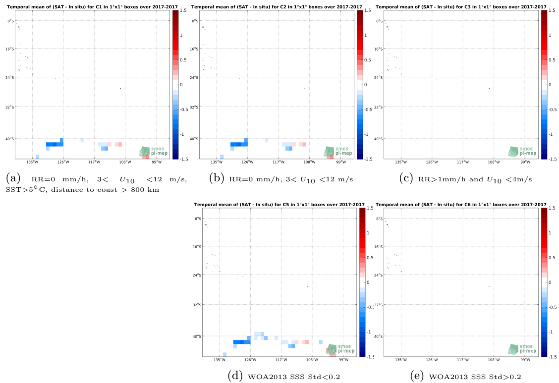
Figure 12: Temporal mean gridded over spatial boxes of size 1^\circ \times 1^\circ of \Delta SSS (SMAP SSS L3 v4 - 8-Day running (RSS) - TSG (GOSUD-Sailing-ship)) for 5 different subdatasets corresponding to: RR=0 mm/h, 3 < U_{10} < 12 m/s, SST > 5^\circ C , distance to coast > 800 km (a), RR=0 mm/h, 3 < U_{10} < 12 m/s (b), RR > 1 mm/h and U_{10} < 4 m/s (c), WOA2013 SSS Std < 0.2 (d), WOA2013 SSS Std > 0.2 (e).
