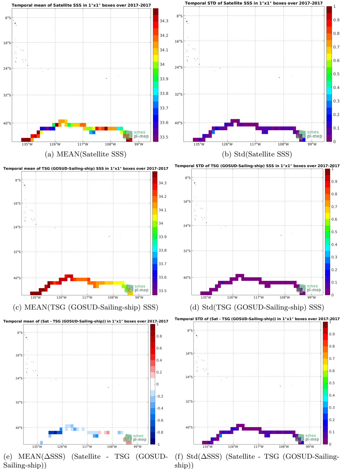
Figure 6: Temporal mean (left) and Std (right) of SSS from SMAP SSS L3 v4 - 8-Day running (RSS) (top), TSG (GOSUD-Sailing-ship) (middle), and of \Delta SSS (Satellite - TSG (GOSUD-Sailing-ship)). Only match-up pairs are used to generate these maps.
