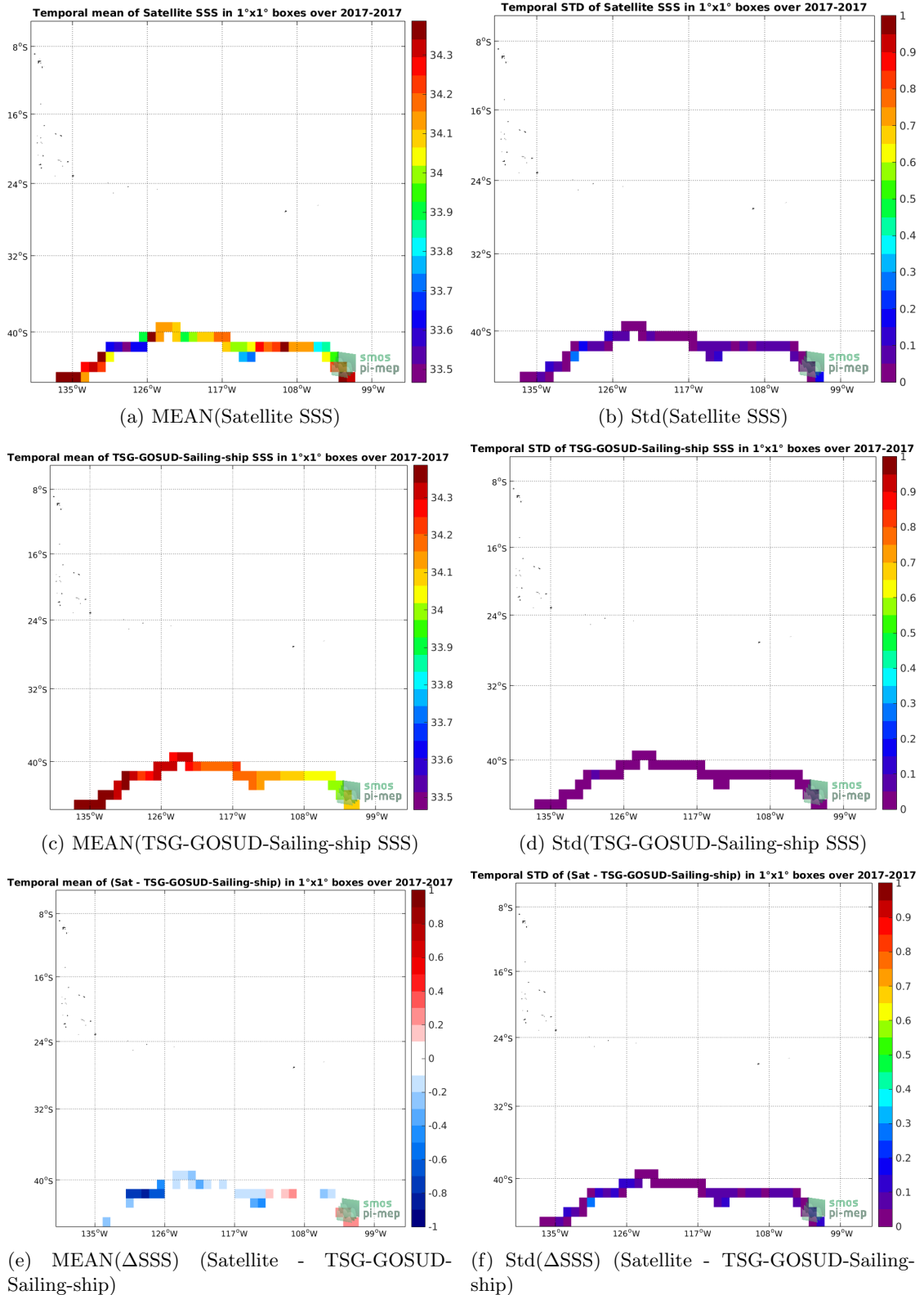
Figure 6: Temporal mean (left) and Std (right) of SSS from SMAP-L3-RSS-V4-8DAY-RUNNING (top), TSG-GOSUD-Sailing-ship (middle), and \Delta SSS (Satellite - TSG-GOSUD-Sailing-ship). Only match-up pairs are used to generate these maps.
