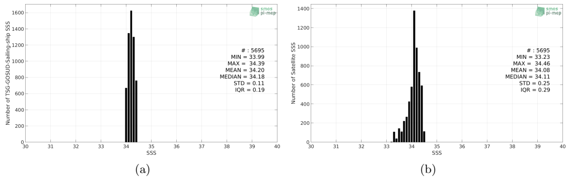
Figure 2: Histograms of SSS from TSG-GOSUD-Sailing-ship (a) and SMAP-L3-RSS-V4-8DAY-RUNNING (b) considering all match-up pairs per bins of 0.1 over the OTT zone Pi-MEP region and for the full satellite product period.
