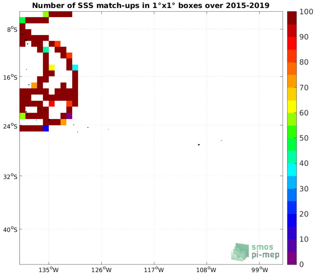
Figure 4: Number of SSS match-ups between TSG (GOSUD-Research-vessel) SSS and the SMAP SSS L3 v4 - 8-Day running (RSS) SSS product for the OTT zone Pi-MEP region over 1°x1° boxes and for the full satellite product period.
