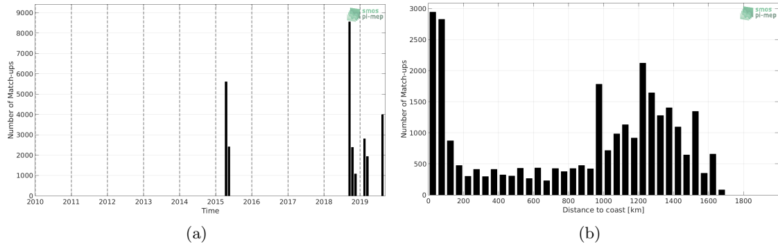
Figure 1: Number of match-ups between TSG (GOSUD-Research-vessel) and SMAP SSS L3 v4 - 8-Day running (RSS) SSS as a function of time (a) and as function of the distance to coast (b) over the OTT zone Pi-MEP region and for the full satellite product period.
