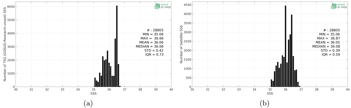
Figure 2: Histograms of SSS from TSG (GOSUD-Research-vessel) (a) and SMAP SSS L3 v4 - 8-Day running (RSS) (b) considering all match-up pairs per bins of 0.1 over the OTT zone Pi-MEP region and for the full satellite product period.
