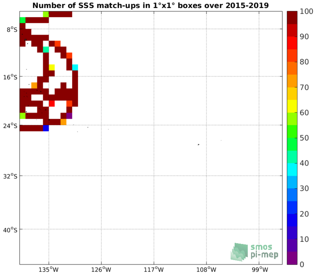
Figure 4: Number of SSS match-ups between TSG (GOSUD-Research-vessel) SSS and the SMAP SSS L3 v4 - 8-Day running (RSS) SSS product for the OTT zone Pi-MEP region over 1^\circ \times 1^\circ boxes and for the full satellite product period.
