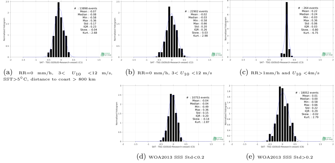
Figure 13: Normalized histogram of \Delta SSS (SMAP SSS L3 v4 - 8-Day running (RSS) - TSG (GOSUD-Research-vessel)) for 5 different subdatasets corresponding to: RR=0 mm/h, 3 < U_{10} < 12 m/s, SST > 5°C, distance to coast > 800 km (a), RR=0 mm/h, 3 < U_{10} < 12 m/s (b), RR > 1mm/h and U_{10} < 4 m/s (c), WOA2013 SSS Std < 0.2 (d), WOA2013 SSS Std > 0.2 (e).
