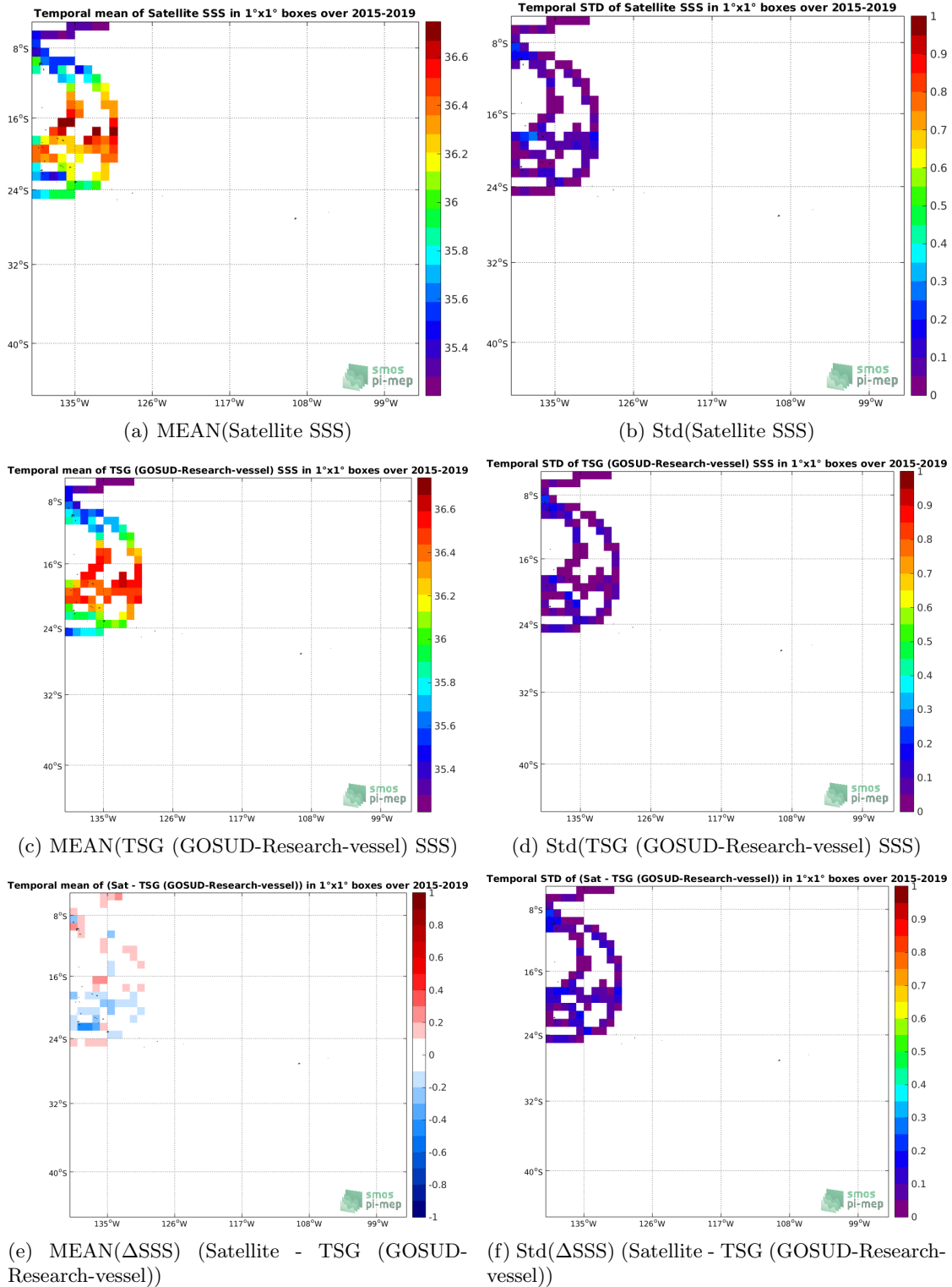
Figure 6: Temporal mean (left) and Std (right) of SSS from SMAP SSS L3 v4 - 8-Day running (RSS) (top), TSG (GOSUD-Research-vessel) (middle), and of \Delta SSS (Satellite - TSG (GOSUD-Research-vessel)). Only match-up pairs are used to generate these maps.
