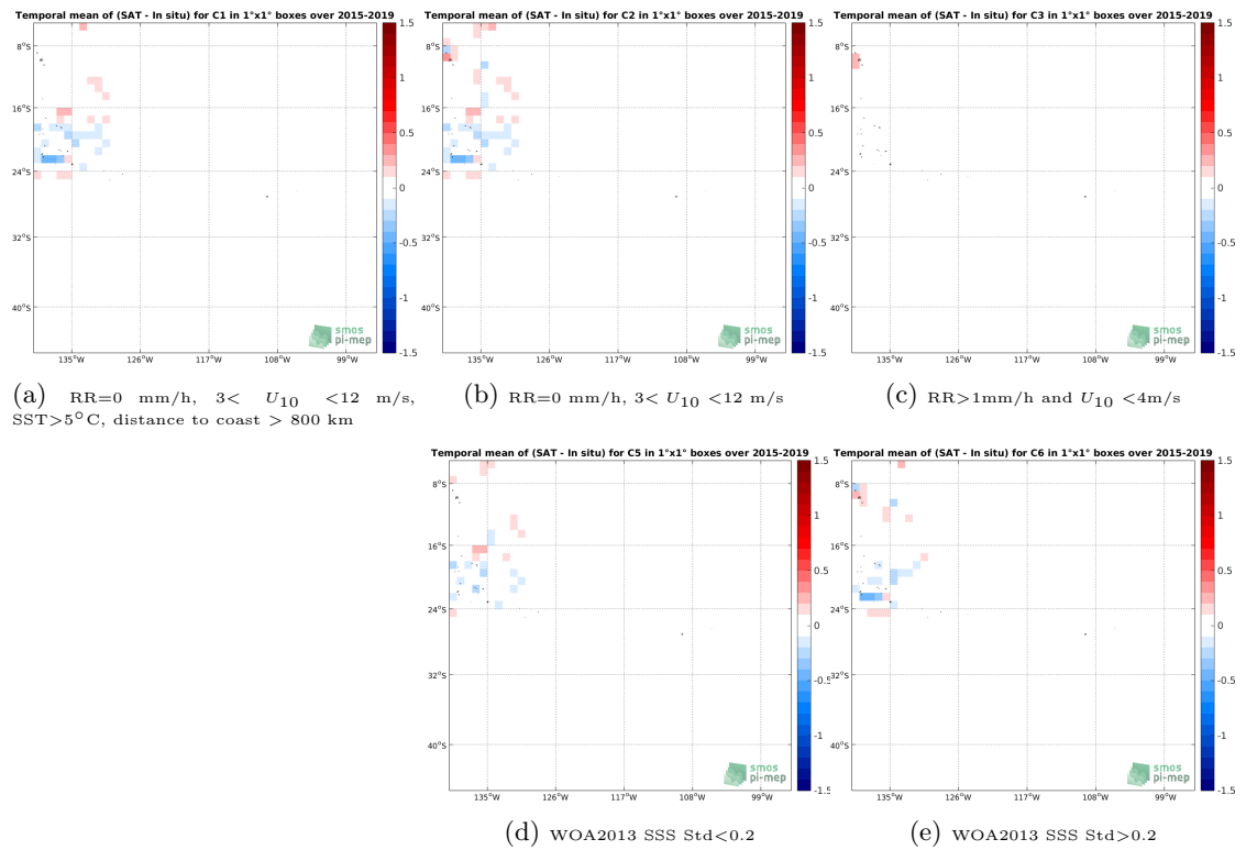
Figure 12: Temporal mean gridded over spatial boxes of size 1^\circ \times 1^\circ of \Delta\text{SSS} (SMAP SSS L3 v4 - 8-Day running (RSS) - TSG (GOSUD-Research-vessel)) for 5 different subdatasets corresponding to:RR=0 mm/h, 3 < U_{10} < 12 m/s, SST>5°C, distance to coast > 800 km (a), RR=0 mm/h, 3 < U_{10} < 12 m/s (b), RR>1mm/h and U_{10} < 4 m/s (c), WOA2013 SSS Std<0.2 (d), WOA2013 SSS Std>0.2 (e).
