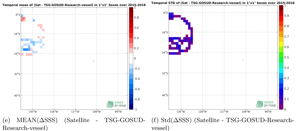
Figure 6: Temporal mean (left) and Std (right) of SSS from SMAP-L3-RSS-V4-8DAY-RUNNING (top), TSG-GOSUD-Research-vessel (middle), and of \Delta SSS (Satellite - TSG-GOSUD-Research-vessel). Only match-up pairs are used to generate these maps.
