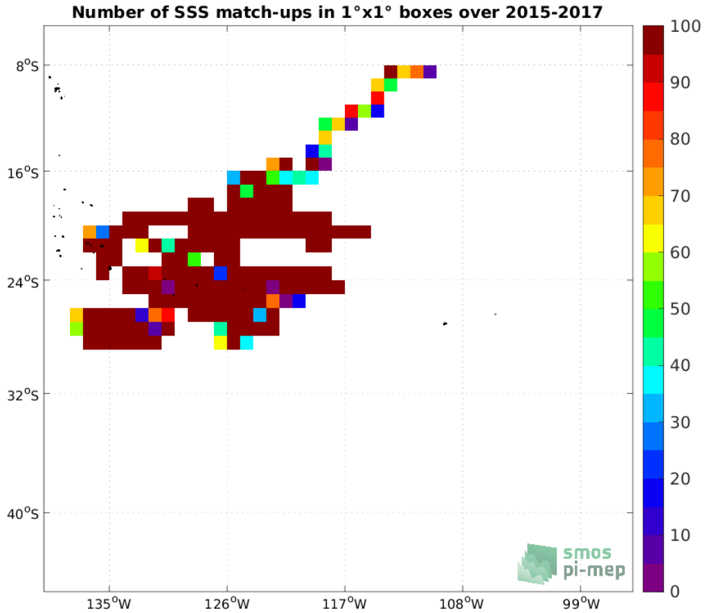
Figure 3: Number of SSS match-ups between Surface drifters SSS and the SMAP SSS L3 v4 - 8-Day running (RSS) SSS product for the OTT zone Pi-MEP region over 1^\circ \times 1^\circ boxes and for the full satellite product period.
