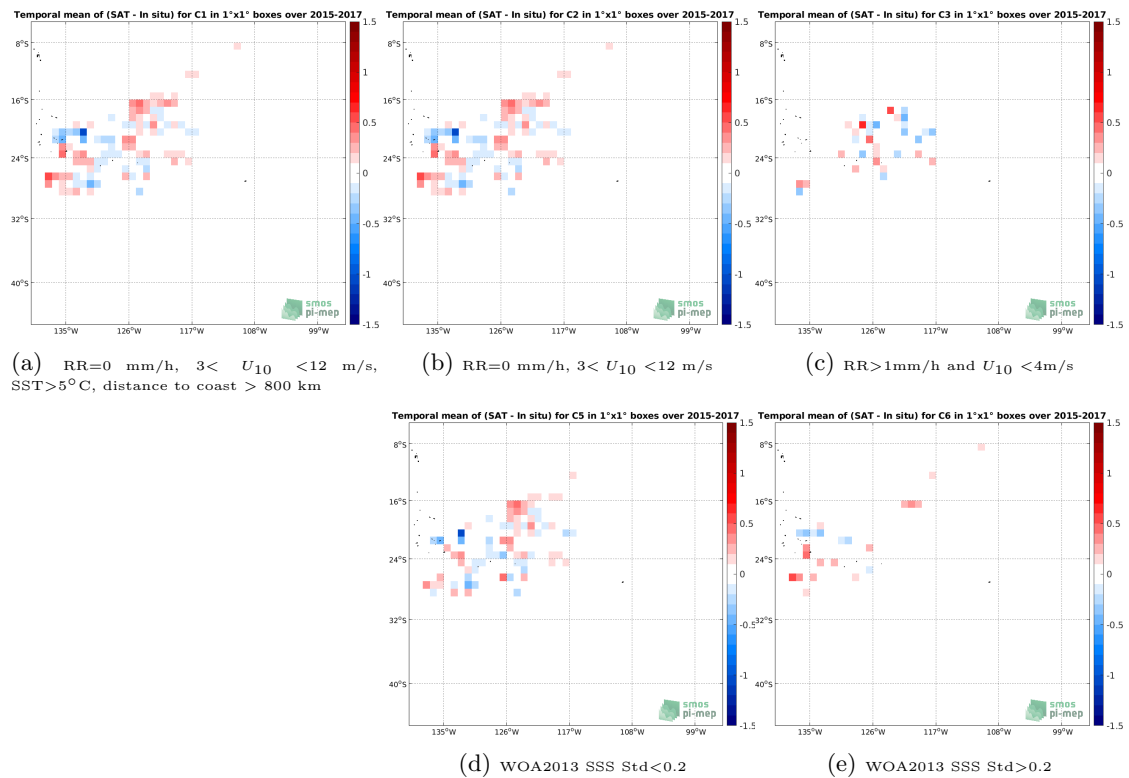
Figure 11: Temporal mean gridded over spatial boxes of size 1^\circ \times 1^\circ of \Delta\text{SSS} (SMAP SSS L3 v4 - 8-Day running (RSS) - Surface drifters) for 5 different subdatasets corresponding to:RR=0 mm/h, 3 < U_{10} < 12 m/s, SST >5^\circ\text{C} , distance to coast > 800 km (a), RR=0 mm/h, 3 < U_{10} < 12 m/s (b), RR >1 mm/h and U_{10} < 4 m/s (c), WOA2013 SSS Std <0.2 (d), WOA2013 SSS Std >0.2 (e).
