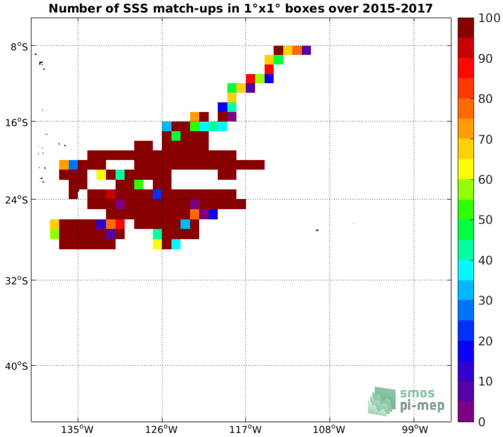
Figure 3: Number of SSS match-ups between Surface drifters SSS and the SMAP SSS L3 v4 - 8-Day running (RSS) SSS product for the OTT zone Pi-MEP region over 1°x1° boxes and for the full satellite product period.
