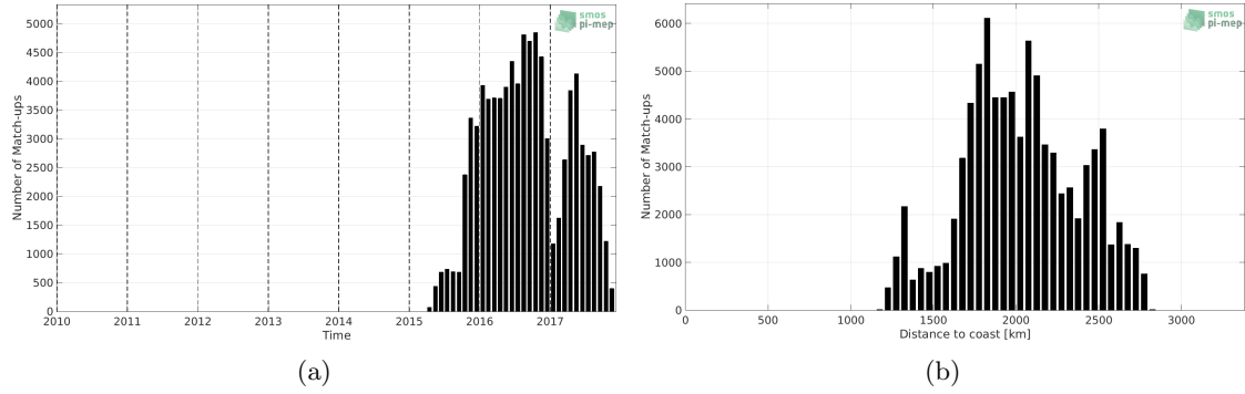
Figure 1: Number of match-ups between Surface drifters and SMAP SSS L3 v4 - 8-Day running (RSS) SSS as a function of time (a) and as function of the distance to coast (b) over the OTT zone Pi-MEP region and for the full satellite product period.
