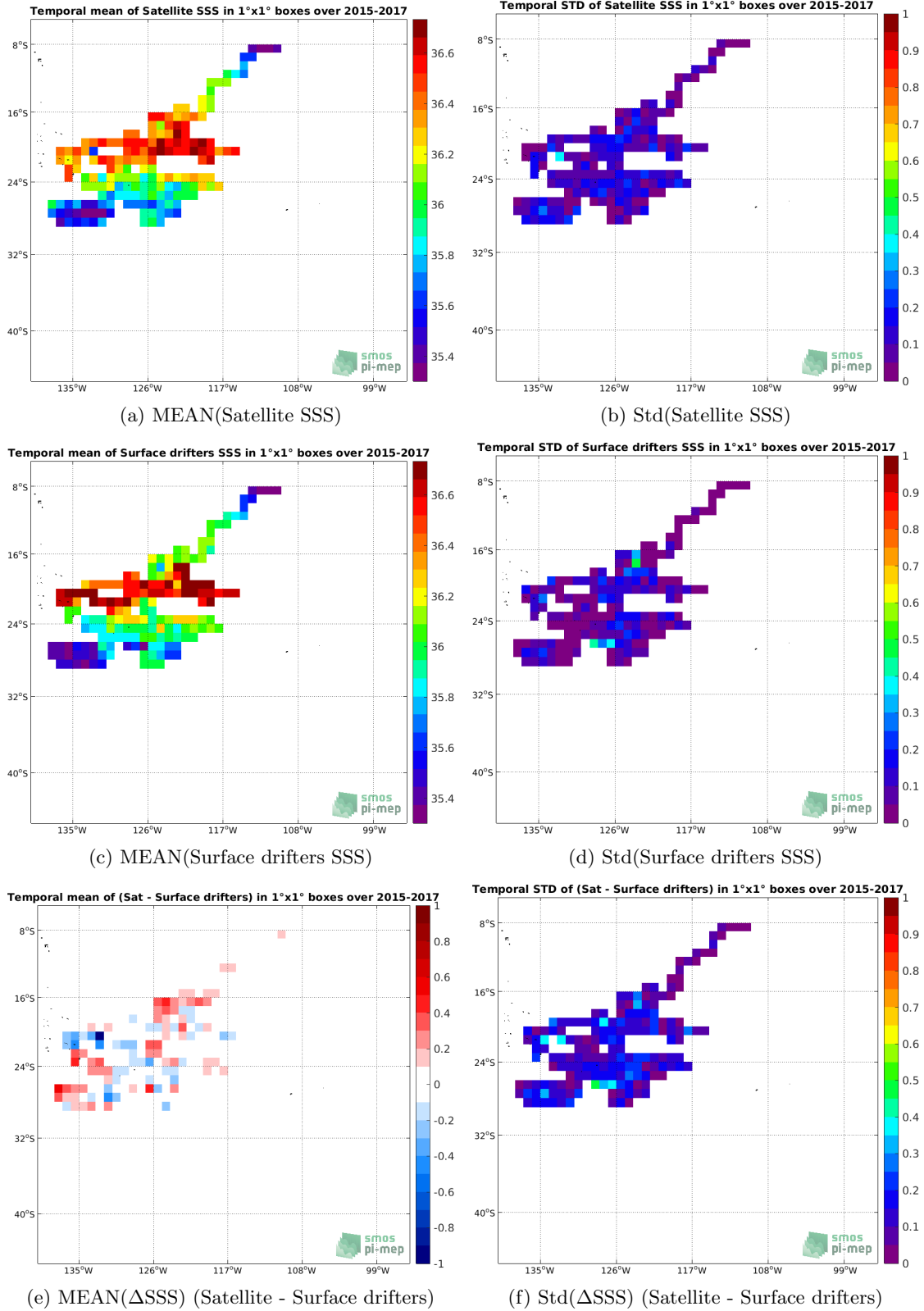
Figure 5: Temporal mean (left) and Std (right) of SSS from SMAP SSS L3 v4 - 8-Day running (RSS) (top), Surface drifters (middle), and of \Delta SSS (Satellite - Surface drifters). Only match-up pairs are used to generate these maps.
