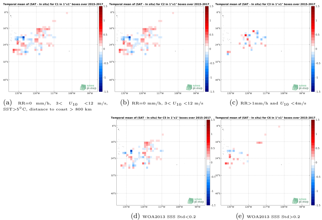
Figure 11: Temporal mean gridded over spatial boxes of size 1^\circ \times 1^\circ of \Delta SSS (SMAP SSS L3 v4 - 8-Day running (RSS) - Surface drifters) for 5 different subdatasets corresponding to:RR=0 mm/h, 3 < U_{10} < 12 m/s, SST > 5^\circ C , distance to coast > 800 km (a), RR=0 mm/h, 3 < U_{10} < 12 m/s (b), RR > 1 mm/h and U_{10} < 4 m/s (c), WOA2013 SSS Std < 0.2 (d), WOA2013 SSS Std > 0.2 (e).
