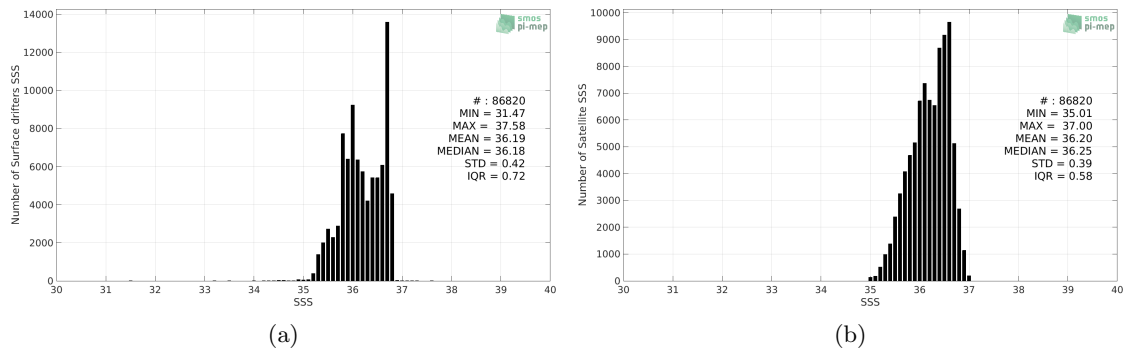
Figure 2: Histograms of SSS from Surface drifters (a) and SMAP SSS L3 v4 - 8-Day running (RSS) (b) considering all match-up pairs per bins of 0.1 over the OTT zone Pi-MEP region and for the full satellite product period.
