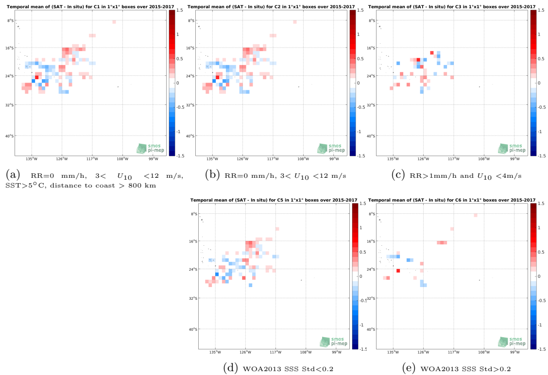
Figure 11: Temporal mean gridded over spatial boxes of size 1^\circ \times 1^\circ of \Delta SSS (SMAP-L3-RSS-V4-8DAY-RUNNING - Surface drifters) for 5 different subdatasets corresponding to:RR=0 mm/h, 3 < U_{10} < 12 m/s, SST >5^\circ\text{C} , distance to coast > 800 km (a), RR=0 mm/h, 3 < U_{10} < 12 m/s (b), RR >1 mm/h and U_{10} < 4 m/s (c), WOA2013 SSS Std <0.2 (d), WOA2013 SSS Std >0.2 (e).
