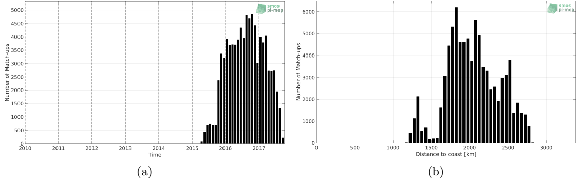
Figure 1: Number of match-ups between Surface drifters and SMAP-L3-RSS-V4-8DAY-RUNNING SSS as a function of time (a) and as function of the distance to coast (b) over the OTT zone Pi-MEP region and for the full satellite product period.
