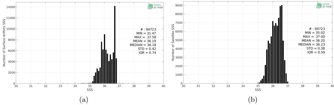
Figure 2: Histograms of SSS from Surface drifters (a) and SMAP-L3-RSS-V4-8DAY-RUNNING (b) considering all match-up pairs per bins of 0.1 over the OTT zone Pi-MEP region and for the full satellite product period.
