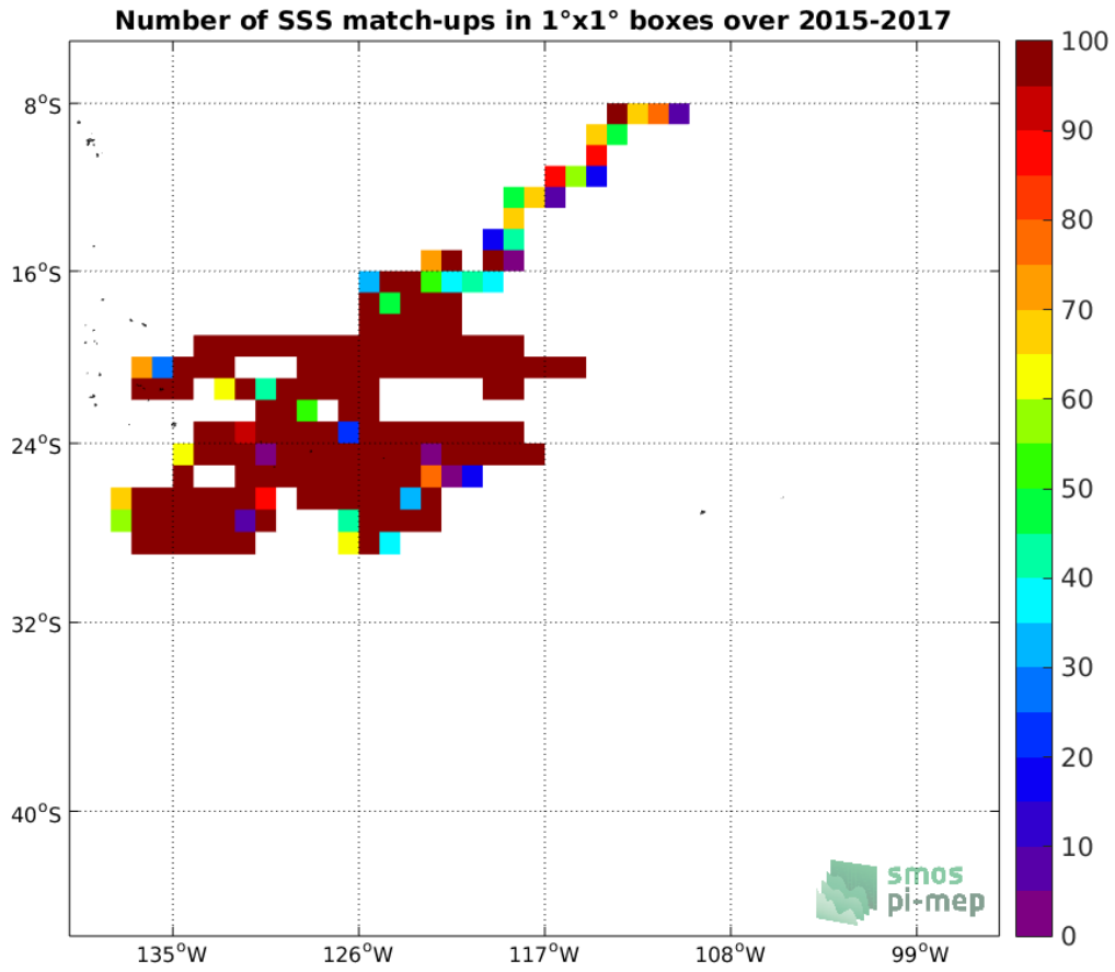
Figure 3: Number of SSS match-ups between Surface drifters SSS and the SMAP-L3-RSS-V4-8DAY-RUNNING SSS product for the OTT zone Pi-MEP region over 1°x1° boxes and for the full satellite product period.
