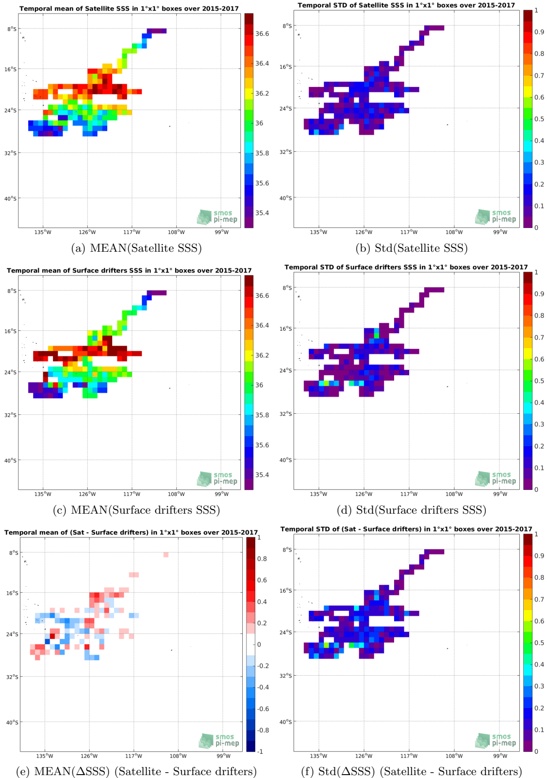
Figure 5: Temporal mean (left) and Std (right) of SSS from SMAP-L3-RSS-V4-8DAY-RUNNING (top), Surface drifters (middle), and of \Delta SSS (Satellite - Surface drifters). Only match-up pairs are used to generate these maps.
