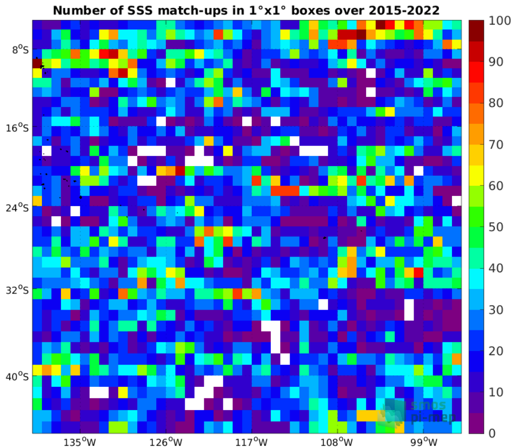
Figure 4: Number of SSS match-ups between Argo SSS and the SMAP SSS L3 v4 - 8-Day running (RSS) SSS product for the OTT zone Pi-MEP region over 1°×1° boxes and for the full satellite product period.
