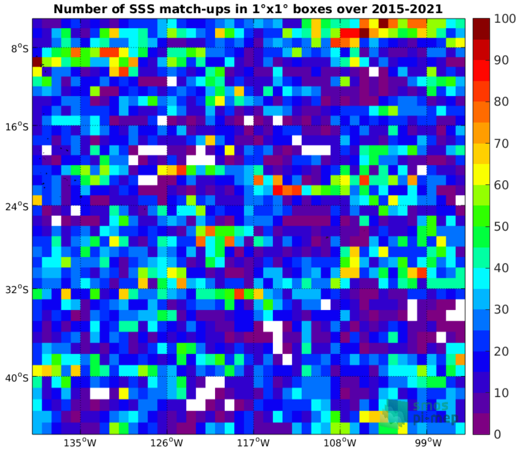
Figure 4: Number of SSS match-ups between Argo SSS and the SMAP SSS L3 v4 - 8-Day running (RSS) SSS product for the OTT zone Pi-MEP region over 1^\circ \times 1^\circ boxes and for the full satellite product period.
