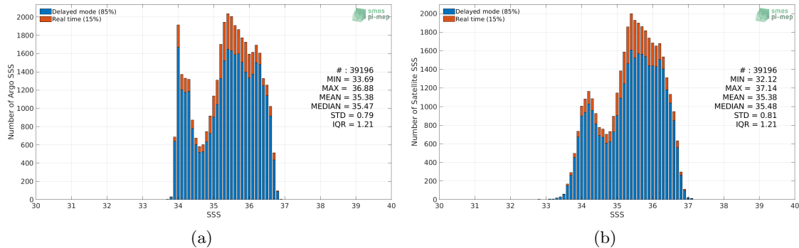
Figure 2: Histograms of SSS from Argo (a) and SMAP SSS L3 v4 - 8-Day running (RSS) (b) considering all match-up pairs per bins of 0.1 over the OTT zone Pi-MEP region and for the full satellite product period.
