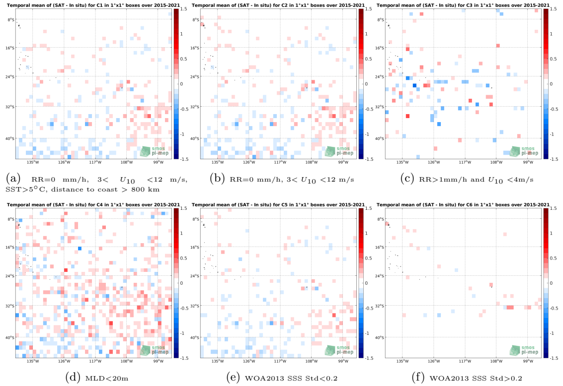
Figure 12: Temporal mean gridded over spatial boxes of size 1^\circ \times 1^\circ of \Delta SSS (SMAP SSS L3 v4 - 8-Day running (RSS) - Argo) for 6 different subdatasets corresponding to:RR=0 mm/h, 3 < U_{10} < 12 m/s, SST >5^\circ C, distance to coast > 800 km (a), RR=0 mm/h, 3 < U_{10} < 12 m/s (b), RR >1 mm/h and U_{10} < 4 m/s (c),MLD <20 m (d),WOA2013 SSS Std <0.2 (e),WOA2013 SSS Std >0.2 (f).
