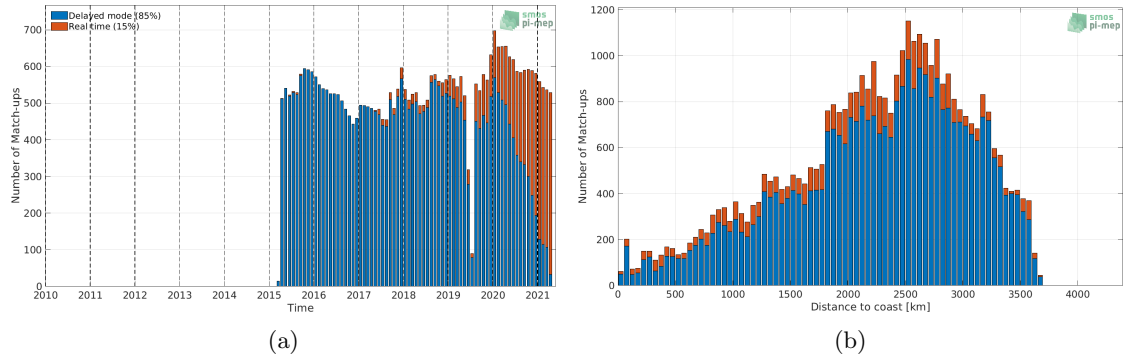
Figure 1: Number of match-ups between Argo and SMAP SSS L3 v4 - 8-Day running (RSS) SSS as a function of time (a) and as function of the distance to coast (b) over the OTT zone Pi-MEP region and for the full satellite product period.
