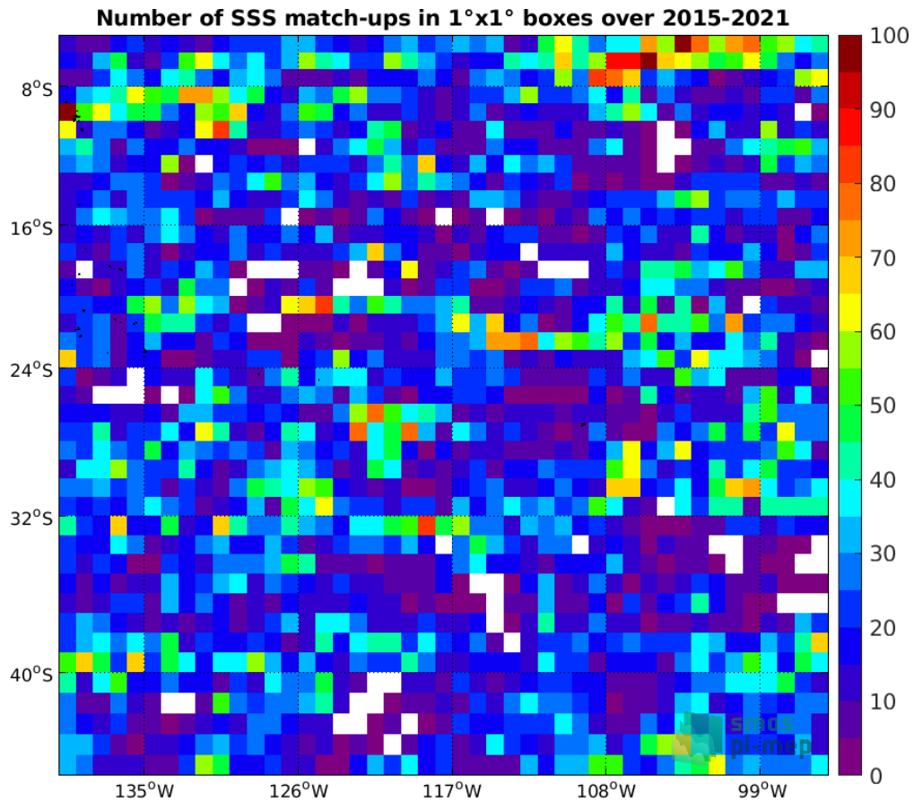
Figure 4: Number of SSS match-ups between Argo SSS and the SMAP SSS L3 v4 - 8-Day running (RSS) SSS product for the OTT zone Pi-MEP region over 1°x1° boxes and for the full satellite product period.
