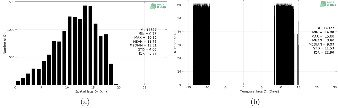
Figure 5: Histograms of the spatial (a) and temporal (b) lags between the location/time of the TSG (SAMOS) measurement and the date of the corresponding SMAP SSS L3 v4 - Monthly (RSS) SSS pixel.
