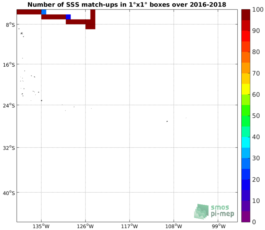
Figure 4: Number of SSS match-ups between TSG (SAMOS) SSS and the SMAP SSS L3 v4 - Monthly (RSS) SSS product for the OTT zone Pi-MEP region over 1^\circ \times 1^\circ boxes and for the full satellite product period.
