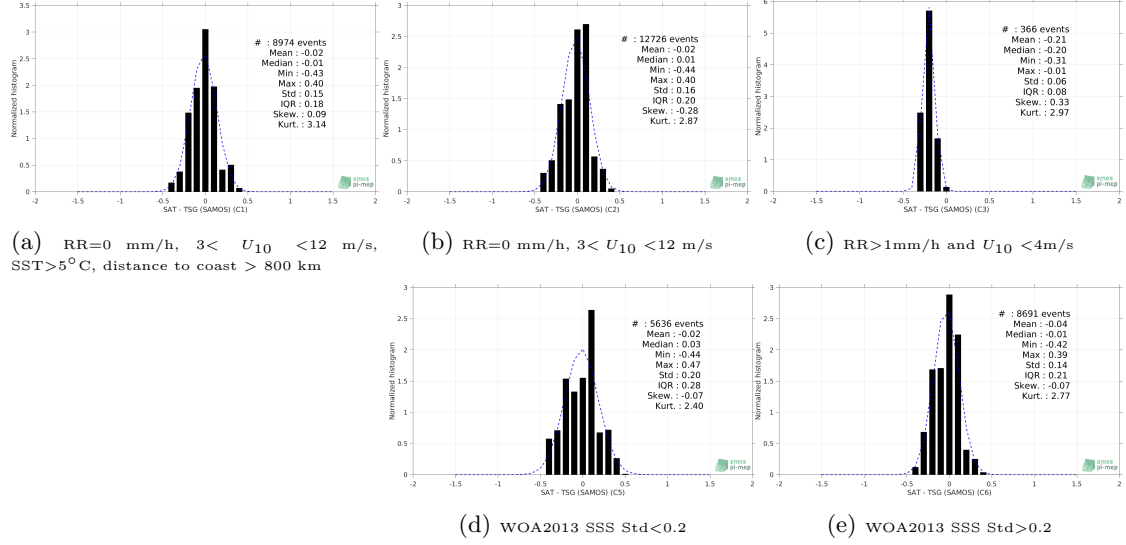
Figure 13: Normalized histogram of \Delta\text{SSS} (SMAP SSS L3 v4 - Monthly (RSS) - TSG (SAMOS)) for 5 different subdatasets corresponding to: \text{RR}=0 \text{ mm/h} , 3 < U_{10} < 12 \text{ m/s} , \text{SST} > 5^\circ\text{C} , distance to coast > 800 \text{ km} (a), \text{RR}=0 \text{ mm/h} , 3 < U_{10} < 12 \text{ m/s} (b), \text{RR} > 1 \text{ mm/h} and U_{10} < 4 \text{ m/s} (c), \text{WOA2013 SSS Std} < 0.2 (d), \text{WOA2013 SSS Std} > 0.2 (e).
