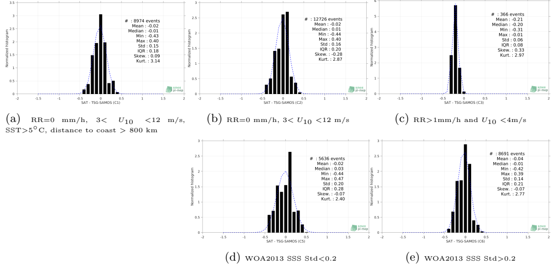
Figure 13: Normalized histogram of \Delta\text{SSS} (SMAP-L3-RSS-V4-MONTHLY - TSG-SAMOS) for 5 different subdatasets corresponding to: RR=0 mm/h, 3 < U_{10} < 12 m/s, SST > 5^\circ\text{C} , distance to coast > 800 km (a), RR=0 mm/h, 3 < U_{10} < 12 m/s (b), RR > 1\text{mm/h} and U_{10} < 4\text{m/s} (c), WOA2013 SSS Std < 0.2 (d), WOA2013 SSS Std > 0.2 (e).
