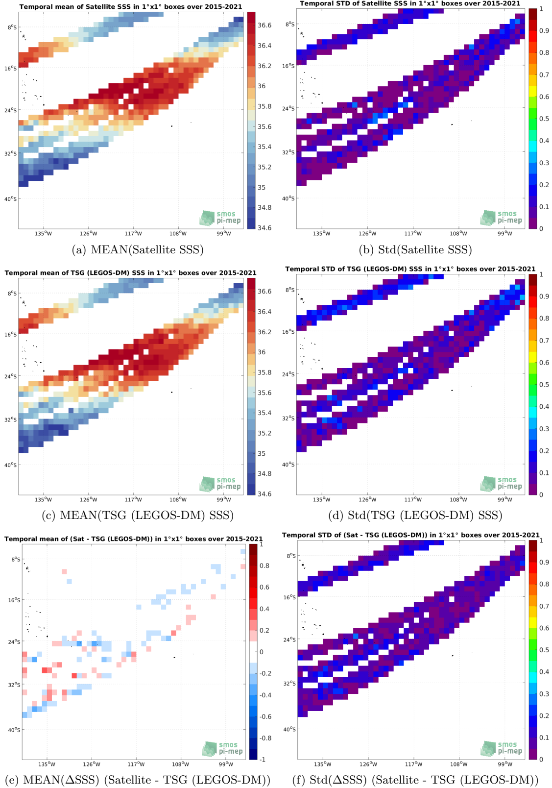
Figure 6: Temporal mean (left) and Std (right), of SSS from SMAP SSS L3 v4 - Monthly (RSS) (top), TSG (LEGOS-DM) (middle), and of \Delta SSS (Satellite - TSG (LEGOS-DM)). Only match-up pairs are used to generate these maps.
