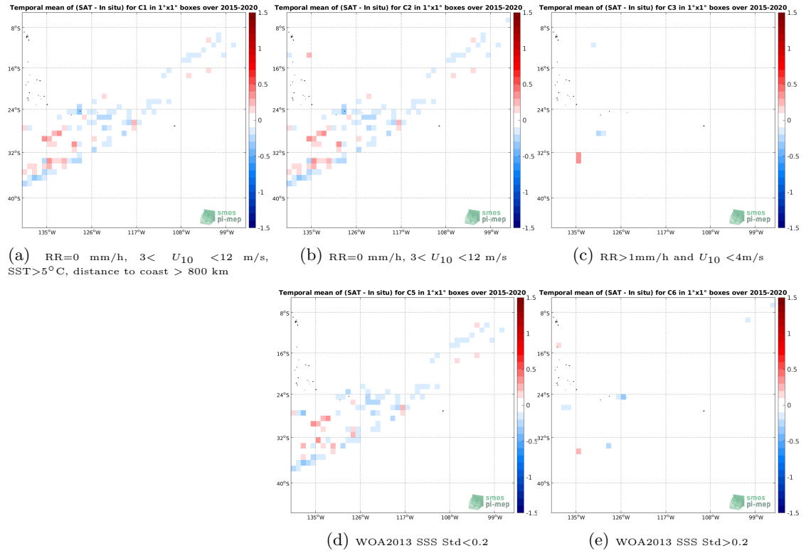
Figure 12: Temporal mean gridded over spatial boxes of size 1^\circ \times 1^\circ of \Delta SSS (SMAP SSS L3 v4 - Monthly (RSS) - TSG (LEGOS-DM)) for 5 different subdatasets corresponding to: RR=0 mm/h, 3 < U_{10} < 12 m/s, SST > 5^\circ C , distance to coast > 800 km (a), RR=0 mm/h, 3 < U_{10} < 12 m/s (b), RR > 1 mm/h and U_{10} < 4 m/s (c), WOA2013 SSS Std < 0.2 (d), WOA2013 SSS Std > 0.2 (e).
