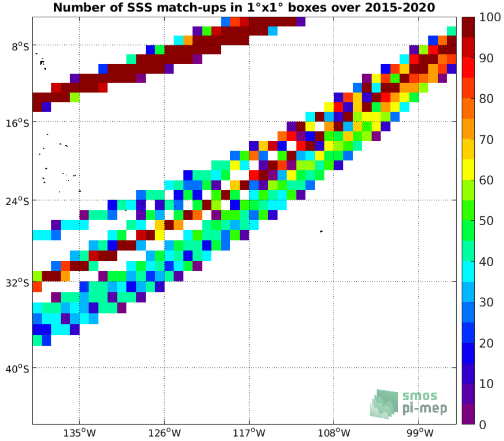
Figure 4: Number of SSS match-ups between TSG (LEGOS-DM) SSS and the SMAP SSS L3 v4 - Monthly (RSS) SSS product for the OTT zone Pi-MEP region over 1°x1° boxes and for the full satellite product period.
