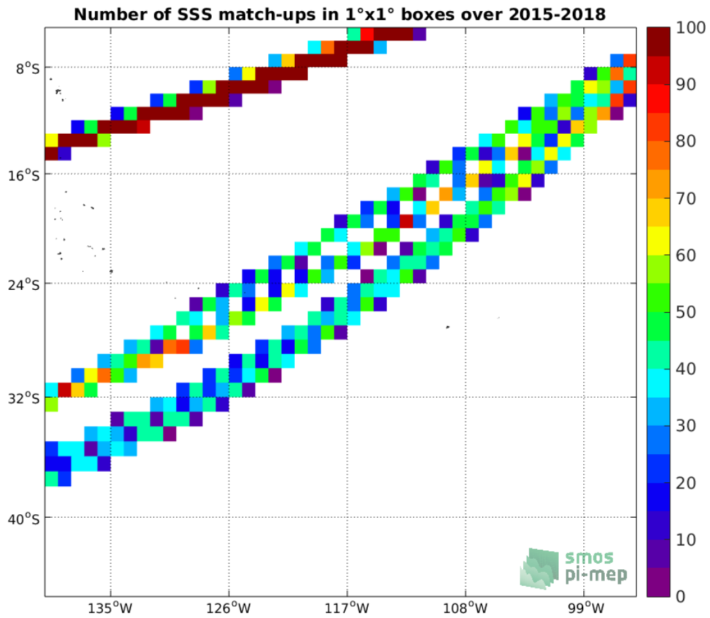
Figure 4: Number of SSS match-ups between TSG-LEGOS-DM SSS and the SMAP-L3-RSS-V4-MONTHLY SSS product for the OTT zone Pi-MEP region over 1°x1° boxes and for the full satellite product period.
