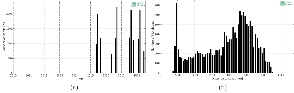
Figure 1: Number of match-ups between TSG-LEGOS-DM and SMAP-L3-RSS-V4-MONTHLY SSS as a function of time (a) and as function of the distance to coast (b) over the OTT zone Pi-MEP region and for the full satellite product period.
