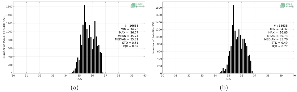
Figure 2: Histograms of SSS from TSG-LEGOS-DM (a) and SMAP-L3-RSS-V4-MONTHLY (b) considering all match-up pairs per bins of 0.1 over the OTT zone Pi-MEP region and for the full satellite product period.
