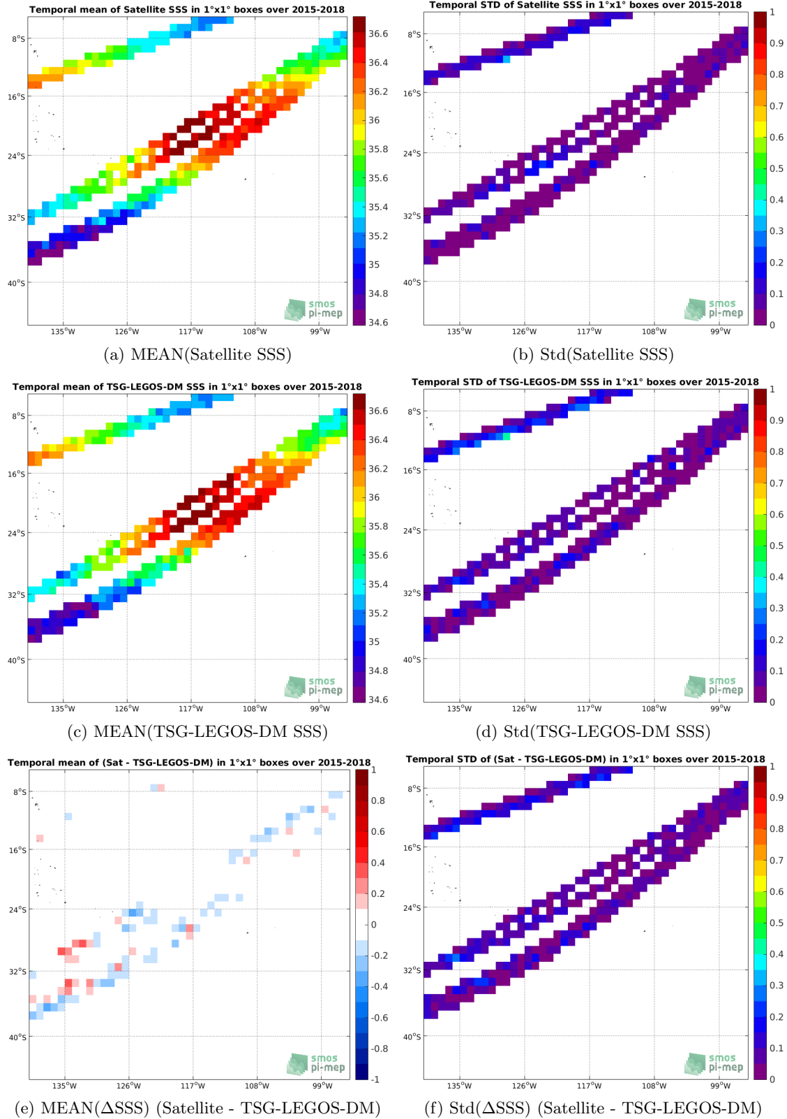
Figure 6: Temporal mean (left) and Std (right) of SSS from SMAP-L3-RSS-V4-MONTHLY (top), TSG-LEGOS-DM (middle), and of \Delta SSS 23 (Satellite - TSG-LEGOS-DM). Only match-up pairs are used to generate these maps.
