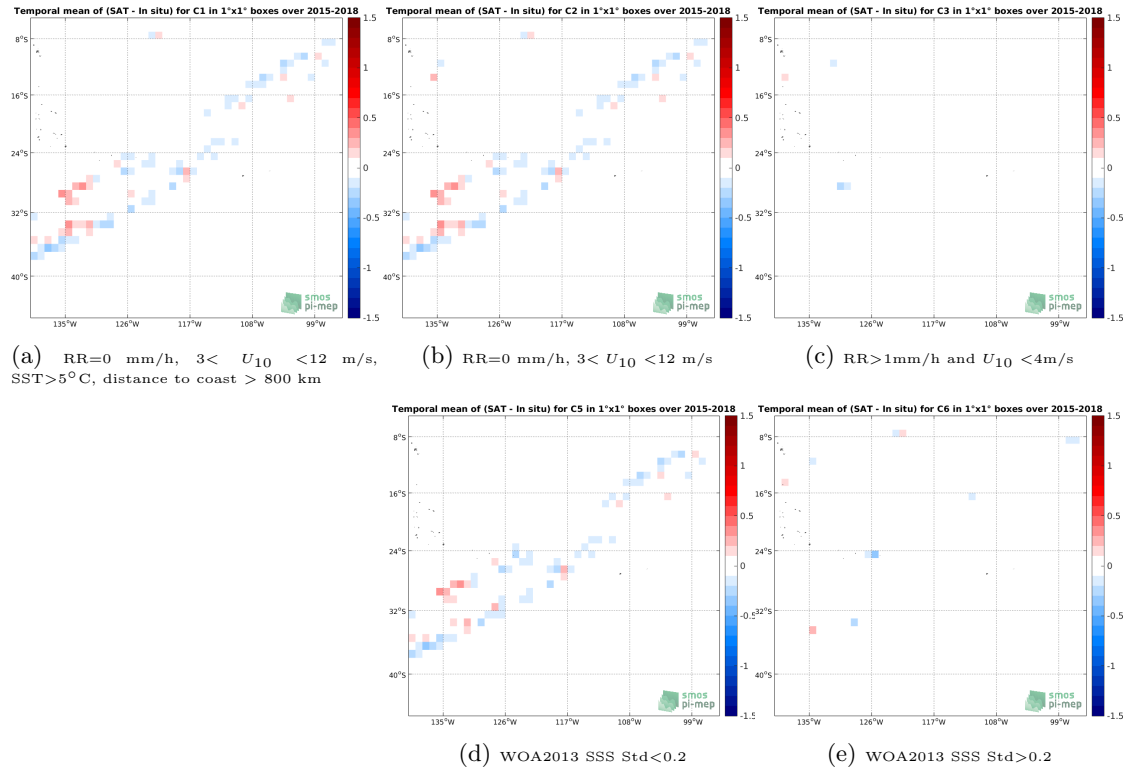
Figure 12: Temporal mean gridded over spatial boxes of size 1^\circ \times 1^\circ of \Delta SSS (SMAP-L3-RSS-V4-MONTHLY - TSG-LEGOS-DM) for 5 different subdatasets corresponding to:RR=0 mm/h, 3 < U_{10} < 12 m/s, SST >5^\circ C, distance to coast > 800 km (a), RR=0 mm/h, 3 < U_{10} < 12 m/s (b), RR >1 mm/h and U_{10} < 4 m/s (c), WOA2013 SSS Std <0.2 (d), WOA2013 SSS Std >0.2 (e).
