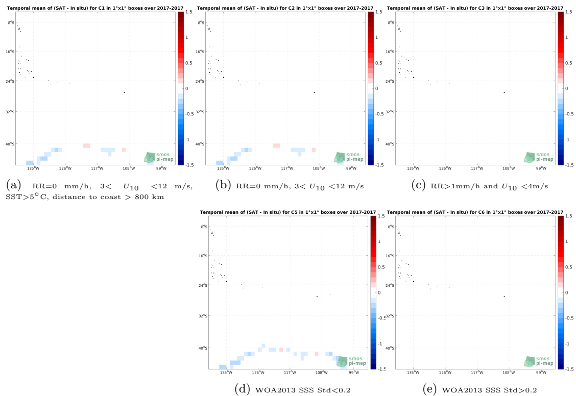
Figure 12: Temporal mean gridded over spatial boxes of size 1^\circ \times 1^\circ of \Delta SSS (SMAP SSS L3 v4 - Monthly (RSS) - TSG (GOSUD-Sailing-ship)) for 5 different subdatasets corresponding to:RR=0 mm/h, 3 < U_{10} < 12 m/s, SST>5°C, distance to coast > 800 km (a), RR=0 mm/h, 3 < U_{10} < 12 m/s (b), RR>1mm/h and U_{10} < 4 m/s (c), WOA2013 SSS Std<0.2 (d), WOA2013 SSS Std>0.2 (e).
