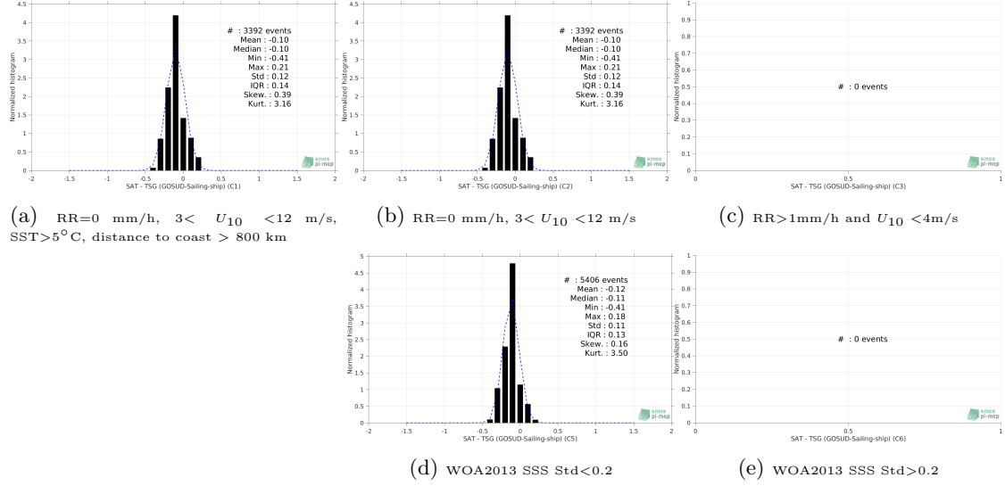
Figure 13: Normalized histogram of \Delta\text{SSS} (SMAP SSS L3 v4 - Monthly (RSS) - TSG (GOSUD-Sailing-ship)) for 5 different subdatasets corresponding to: RR=0 mm/h, 3 < U_{10} < 12 m/s, SST > 5^\circ\text{C} , distance to coast > 800 km (a), RR=0 mm/h, 3 < U_{10} < 12 m/s (b), RR > 1\text{mm/h} and U_{10} < 4\text{m/s} (c), WOA2013 SSS Std < 0.2 (d), WOA2013 SSS Std > 0.2 (e).
