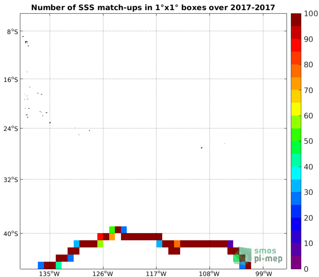
Figure 4: Number of SSS match-ups between TSG (GOSUD-Sailing-ship) SSS and the SMAP SSS L3 v4 - Monthly (RSS) SSS product for the OTT zone Pi-MEP region over 1°x1° boxes and for the full satellite product period.
