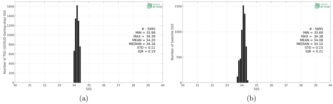
Figure 2: Histograms of SSS from TSG (GOSUD-Sailing-ship) (a) and SMAP SSS L3 v4 - Monthly (RSS) (b) considering all match-up pairs per bins of 0.1 over the OTT zone Pi-MEP region and for the full satellite product period.
