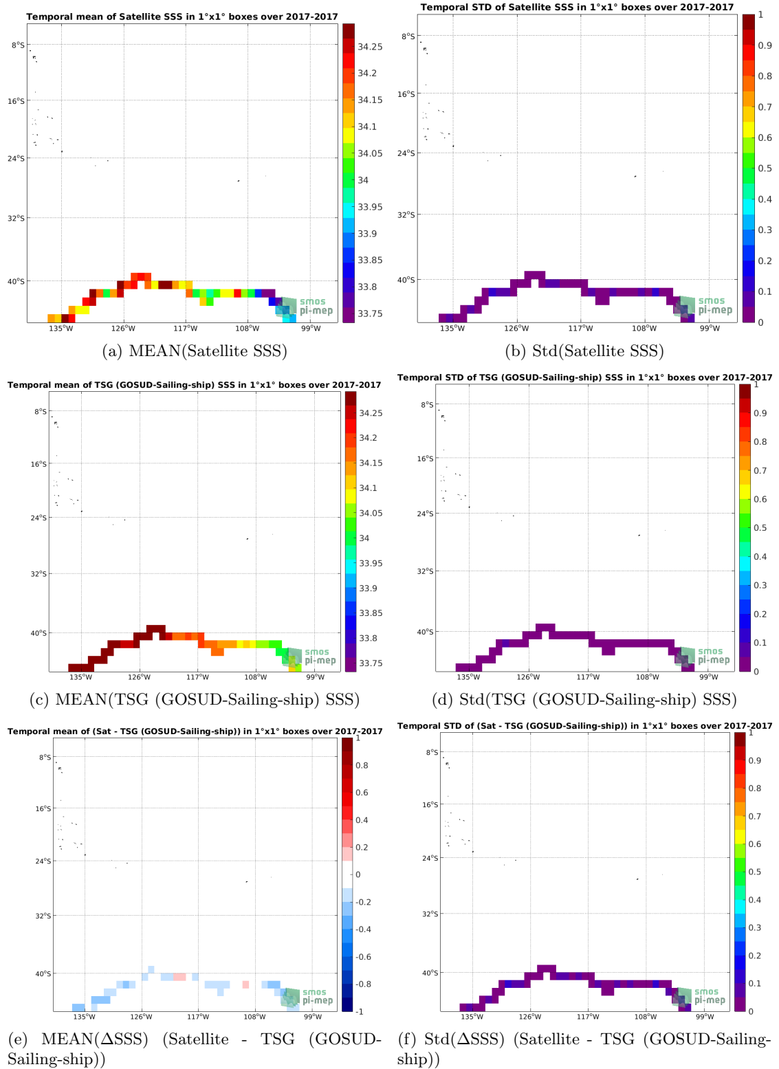
Figure 6: Temporal mean (left) and Std (right) of SSS from SMAP SSS L3 v4 - Monthly (RSS) (top), TSG (GOSUD-Sailing-ship) (middle), and of \Delta SSS (Satellite - TSG (GOSUD-Sailing-ship)). Only match-up pairs are used to generate these maps.
