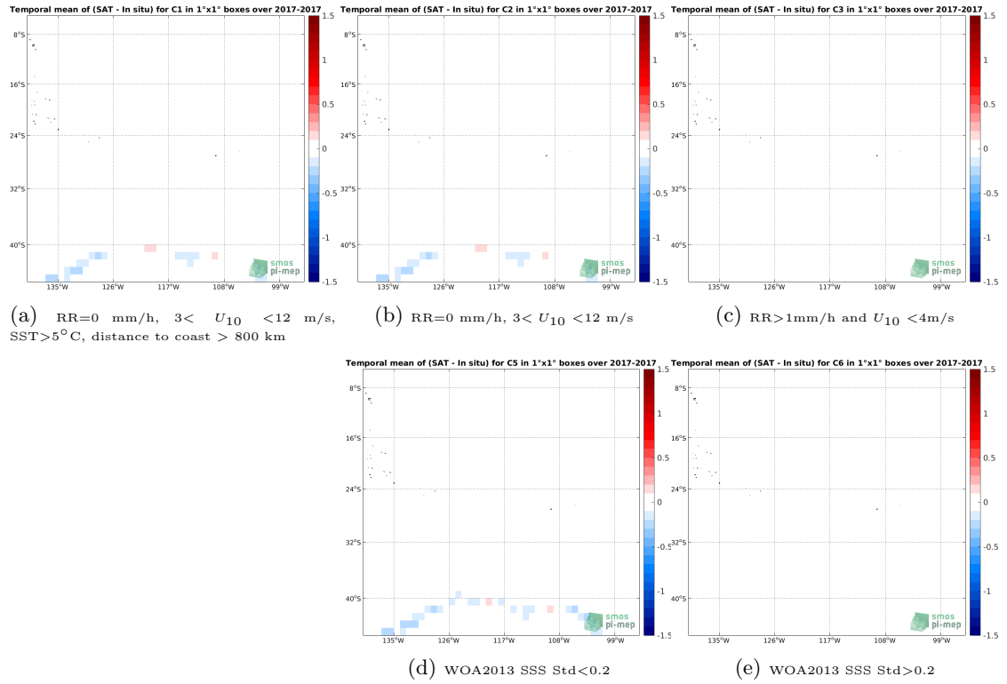
Figure 12: Temporal mean gridded over spatial boxes of size 1^\circ \times 1^\circ of \Delta SSS (SMAP SSS L3 v4 - Monthly (RSS) - TSG (GOSUD-Sailing-ship)) for 5 different subdatasets corresponding to: RR=0 mm/h, 3 < U_{10} < 12 m/s, SST > 5^\circ C , distance to coast > 800 km (a), RR=0 mm/h, 3 < U_{10} < 12 m/s (b), RR > 1 mm/h and U_{10} < 4 m/s (c), WOA2013 SSS Std < 0.2 (d), WOA2013 SSS Std > 0.2 (e).
