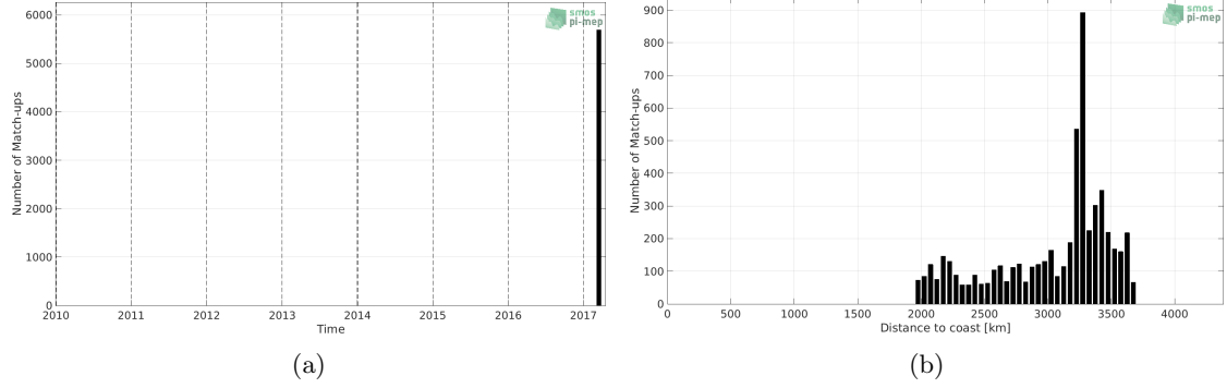
Figure 1: Number of match-ups between TSG (GOSUD-Sailing-ship) and SMAP SSS L3 v4 - Monthly (RSS) SSS as a function of time (a) and as function of the distance to coast (b) over the OTT zone Pi-MEP region and for the full satellite product period.
