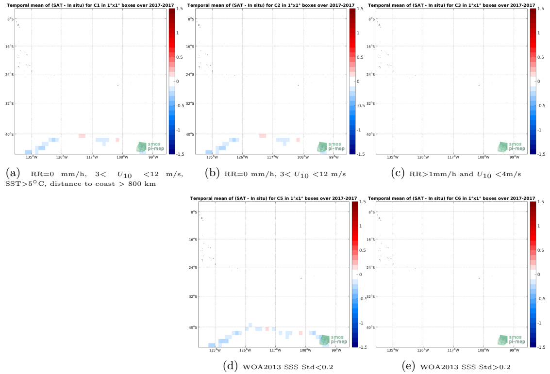
Figure 12: Temporal mean gridded over spatial boxes of size 1^\circ \times 1^\circ of \Delta SSS (SMAP-L3-RSS-V4-MONTHLY - TSG-GOSUD-Sailing-ship) for 5 different subdatasets corresponding to: RR=0 mm/h, 3 < U_{10} < 12 m/s, SST >5^\circ\text{C} , distance to coast > 800 km (a), RR=0 mm/h, 3 < U_{10} < 12 m/s (b), RR >1 mm/h and U_{10} < 4 m/s (c), WOA2013 SSS Std <0.2 (d), WOA2013 SSS Std >0.2 (e).
