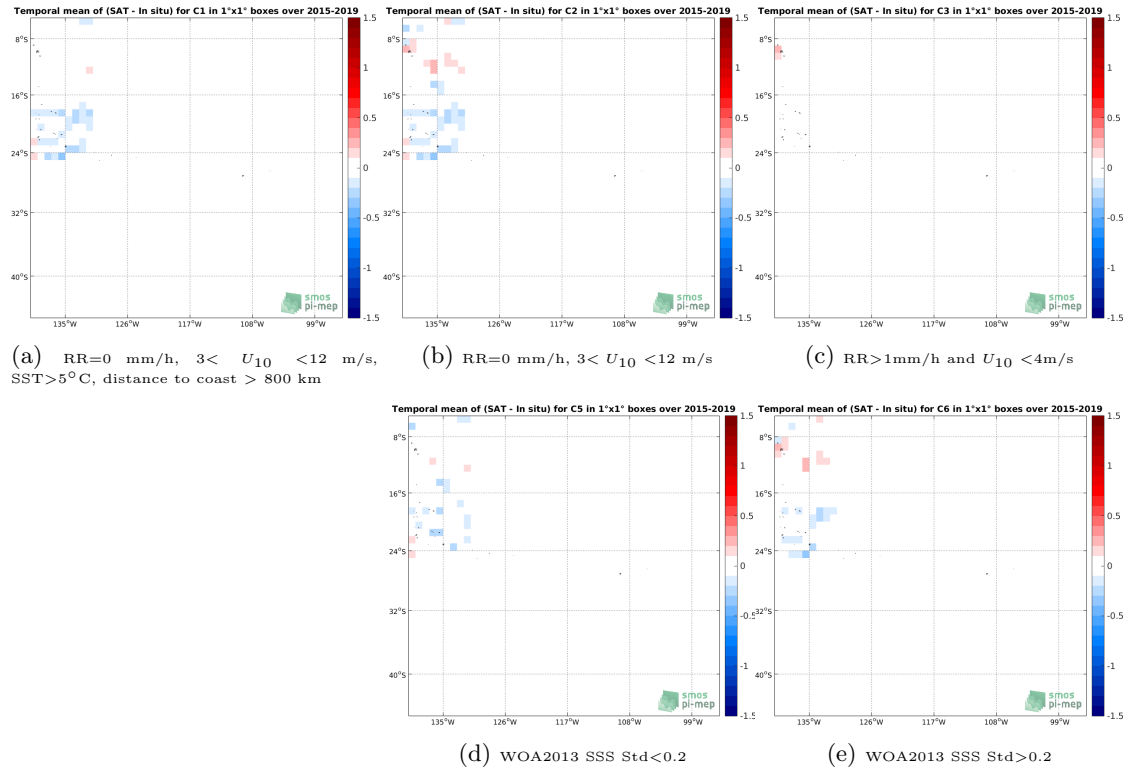
Figure 12: Temporal mean gridded over spatial boxes of size 1^\circ \times 1^\circ of \Delta SSS (SMAP SSS L3 v4 - Monthly (RSS) - TSG (GOSUD-Research-vessel)) for 5 different subdatasets corresponding to: RR=0 mm/h, 3 < U_{10} < 12 m/s, SST >5^\circ C, distance to coast > 800 km (a), RR=0 mm/h, 3 < U_{10} < 12 m/s (b), RR >1 mm/h and U_{10} < 4 m/s (c), WOA2013 SSS Std <0.2 (d), WOA2013 SSS Std >0.2 (e).
