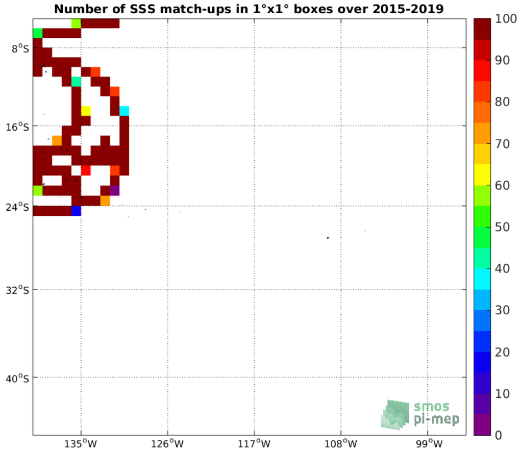
Figure 4: Number of SSS match-ups between TSG (GOSUD-Research-vessel) SSS and the SMAP SSS L3 v4 - Monthly (RSS) SSS product for the OTT zone Pi-MEP region over 1°x1° boxes and for the full satellite product period.
