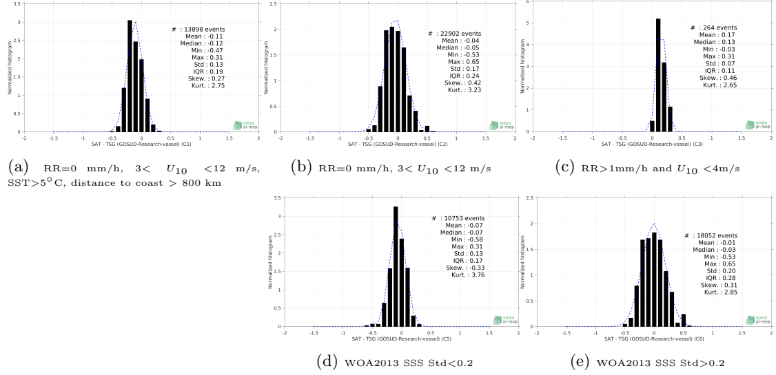
Figure 13: Normalized histogram of \Delta\text{SSS} (SMAP SSS L3 v4 - Monthly (RSS) - TSG (GOSUD-Research-vessel)) for 5 different subdatasets corresponding to: RR=0 mm/h, 3 < U_{10} < 12 m/s, SST > 5^{\circ}\text{C} , distance to coast > 800 km (a), RR=0 mm/h, 3 < U_{10} < 12 m/s (b), RR > 1\text{mm/h} and U_{10} < 4\text{m/s} (c), WOA2013 SSS Std < 0.2 (d), WOA2013 SSS Std > 0.2 (e).
