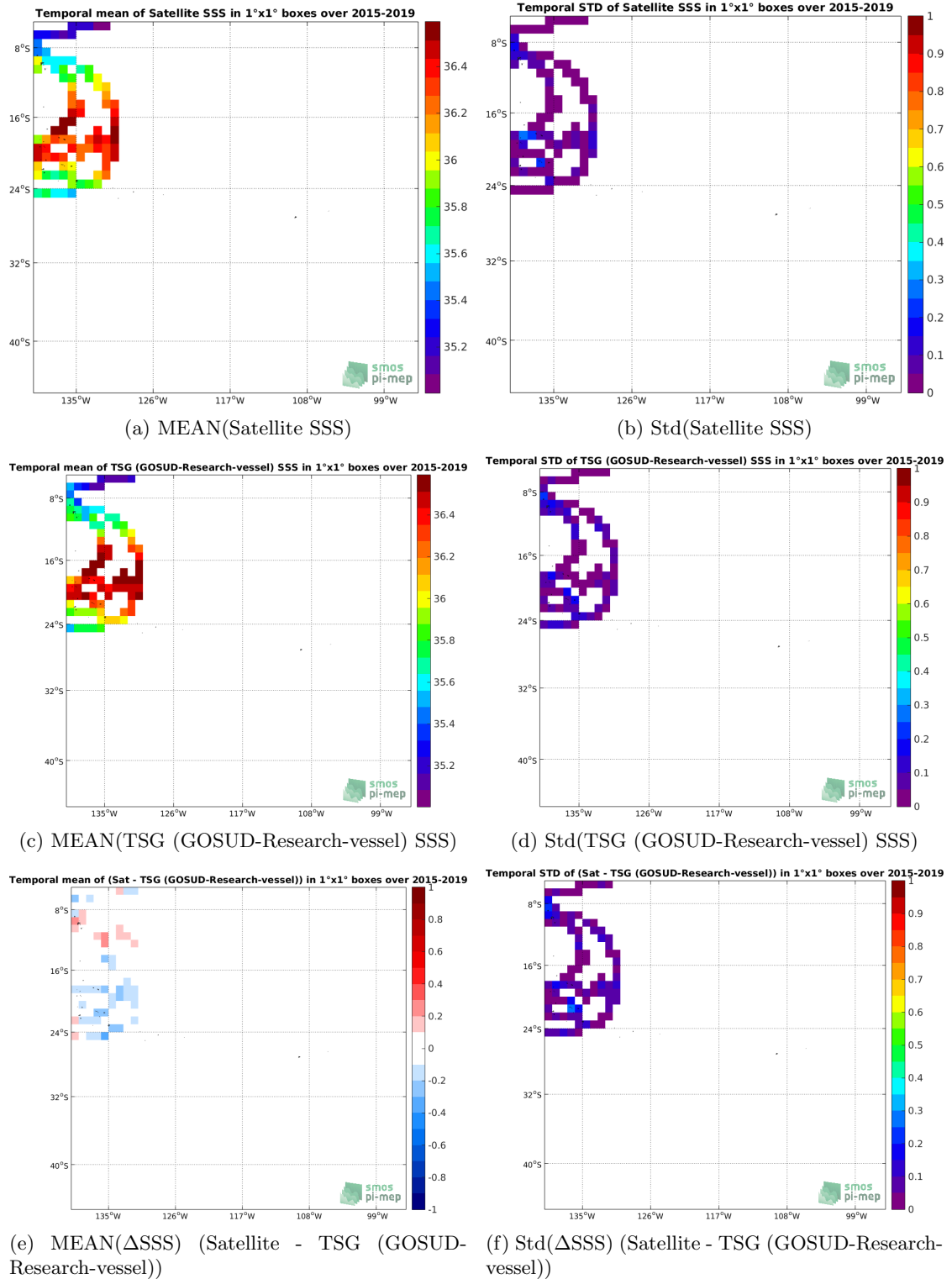
Figure 6: Temporal mean (left) and Std (right) of SSS from SMAP SSS L3 v4 - Monthly (RSS) (top), TSG (GOSUD-Research-vessel) (middle), and of \Delta SSS (Satellite - TSG (GOSUD-Research-vessel)). Only match-up pairs are used to generate these maps.
