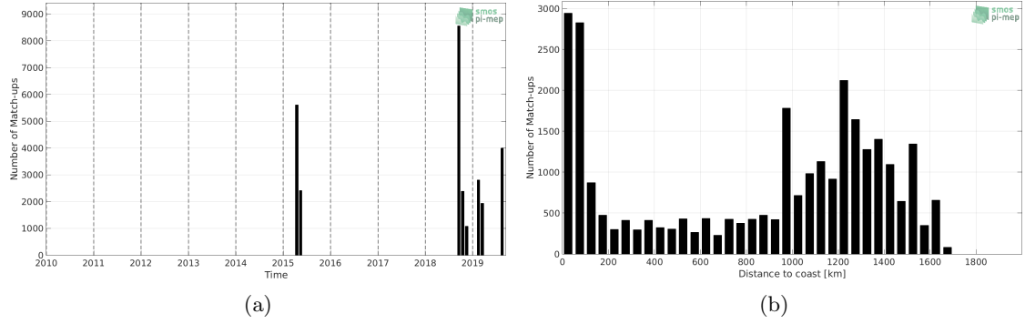
Figure 1: Number of match-ups between TSG (GOSUD-Research-vessel) and SMAP SSS L3 v4 - Monthly (RSS) SSS as a function of time (a) and as function of the distance to coast (b) over the OTT zone Pi-MEP region and for the full satellite product period.
