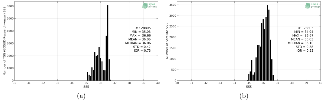
Figure 2: Histograms of SSS from TSG (GOSUD-Research-vessel) (a) and SMAP SSS L3 v4 - Monthly (RSS) (b) considering all match-up pairs per bins of 0.1 over the OTT zone Pi-MEP region and for the full satellite product period.
