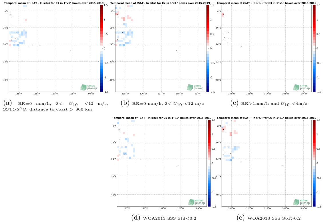
Figure 12: Temporal mean gridded over spatial boxes of size 1^\circ \times 1^\circ of \Delta SSS (SMAP SSS L3 v4 - Monthly (RSS) - TSG (GOSUD-Research-vessel)) for 5 different subdatasets corresponding to: RR=0 mm/h, 3 < U_{10} < 12 m/s, SST > 5^\circ C , distance to coast > 800 km (a), RR=0 mm/h, 3 < U_{10} < 12 m/s (b), RR > 1 mm/h and U_{10} < 4 m/s (c), WOA2013 SSS Std < 0.2 (d), WOA2013 SSS Std > 0.2 (e).
