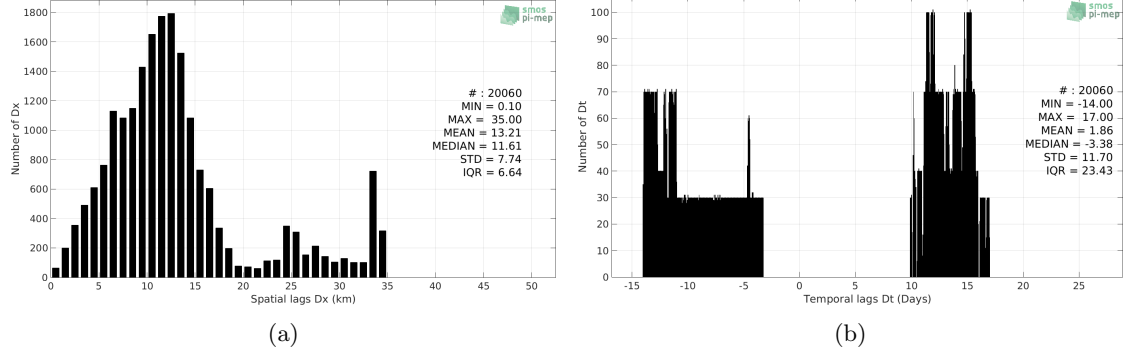
Figure 5: Histograms of the spatial (a) and temporal (b) lags between the time of the TSG-GOSUD-Research-vessel measurements and the date of the corresponding SMAP-L3-RSS-V4-MONTHLY SSS product.
