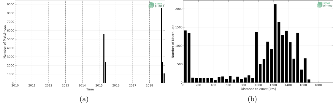
Figure 1: Number of match-ups between TSG-GOSUD-Research-vessel and SMAP-L3-RSS-V4-MONTHLY SSS as a function of time (a) and as function of the distance to coast (b) over the OTT zone Pi-MEP region and for the full satellite product period.
