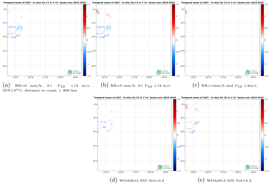
Figure 12: Temporal mean gridded over spatial boxes of size 1^\circ \times 1^\circ of \Delta SSS (SMAP-L3-RSS-V4-MONTHLY - TSG-GOSUD-Research-vessel) for 5 different subdatasets corresponding to:RR=0 mm/h, 3 < U_{10} < 12 m/s, SST >5^\circ C, distance to coast > 800 km (a), RR=0 mm/h, 3 < U_{10} < 12 m/s (b), RR >1 mm/h and U_{10} < 4 m/s (c), WOA2013 SSS Std <0.2 (d), WOA2013 SSS Std >0.2 (e).
