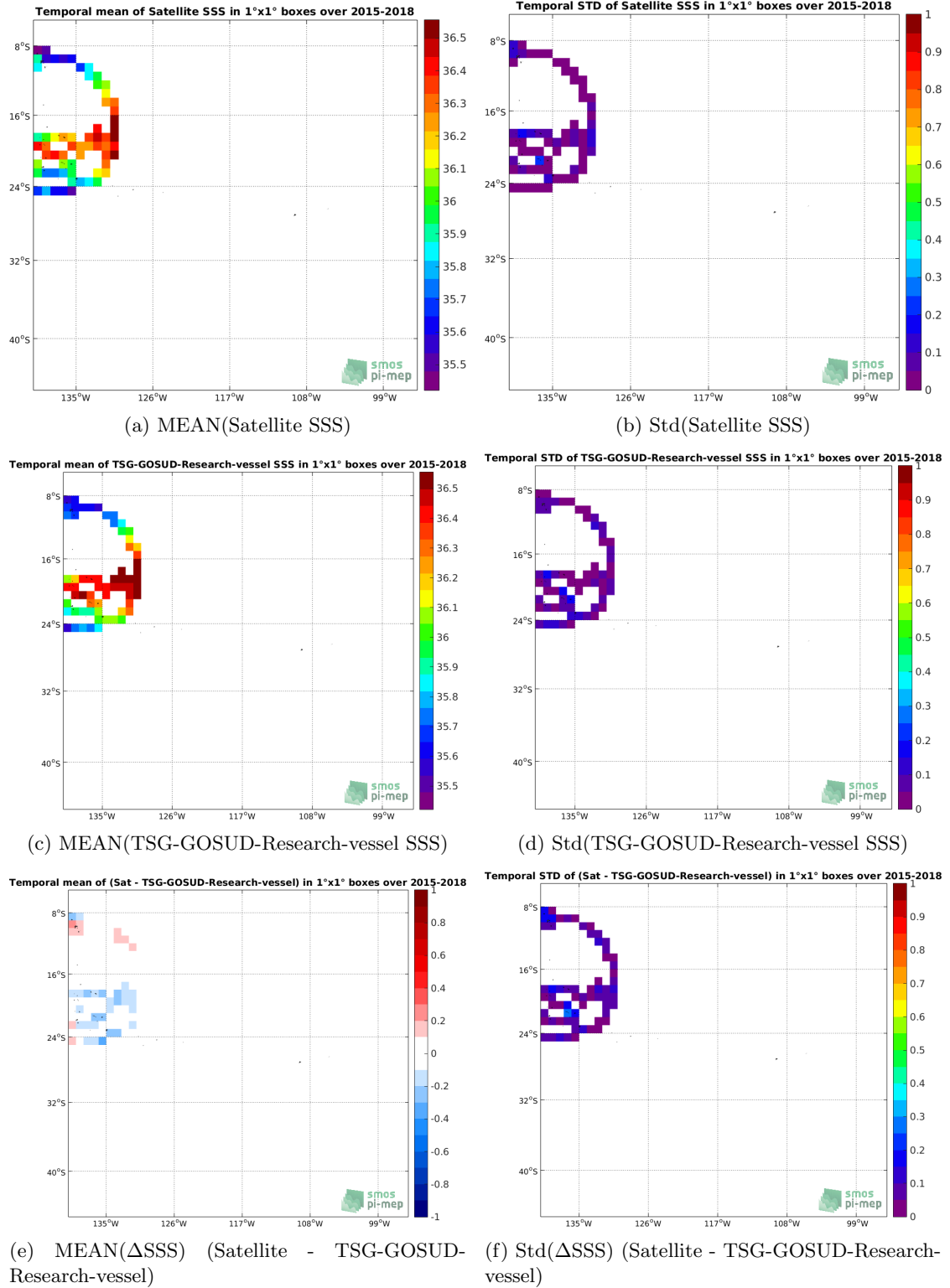
Figure 6: Temporal mean (left) and Std (right) of SSS from SMAP-L3-RSS-V4-MONTHLY (top), TSG-GOSUD-Research-vessel (middle), and of \Delta SSS (Satellite - TSG-GOSUD-Research-vessel). Only match-up pairs are used to generate these maps.
