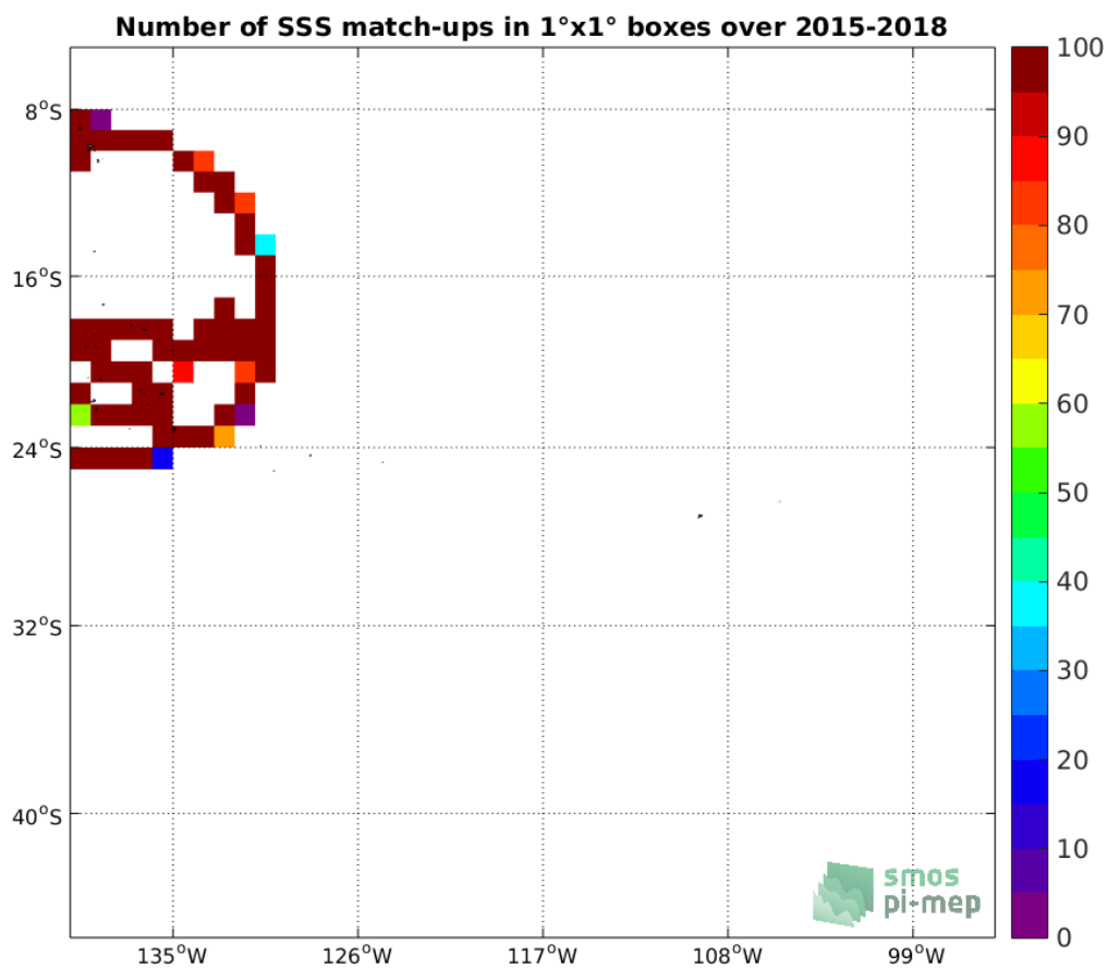
Figure 4: Number of SSS match-ups between TSG-GOSUD-Research-vessel SSS and the SMAP-L3-RSS-V4-MONTHLY SSS product for the OTT zone Pi-MEP region over 1°x1° boxes and for the full satellite product period.
