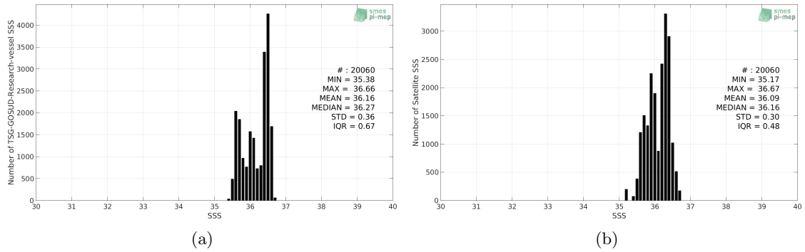
Figure 2: Histograms of SSS from TSG-GOSUD-Research-vessel (a) and SMAP-L3-RSS-V4-MONTHLY (b) considering all match-up pairs per bins of 0.1 over the OTT zone Pi-MEP region and for the full satellite product period.
