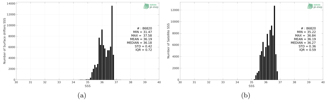
Figure 2: Histograms of SSS from Surface drifters (a) and SMAP SSS L3 v4 - Monthly (RSS) (b) considering all match-up pairs per bins of 0.1 over the OTT zone Pi-MEP region and for the full satellite product period.
