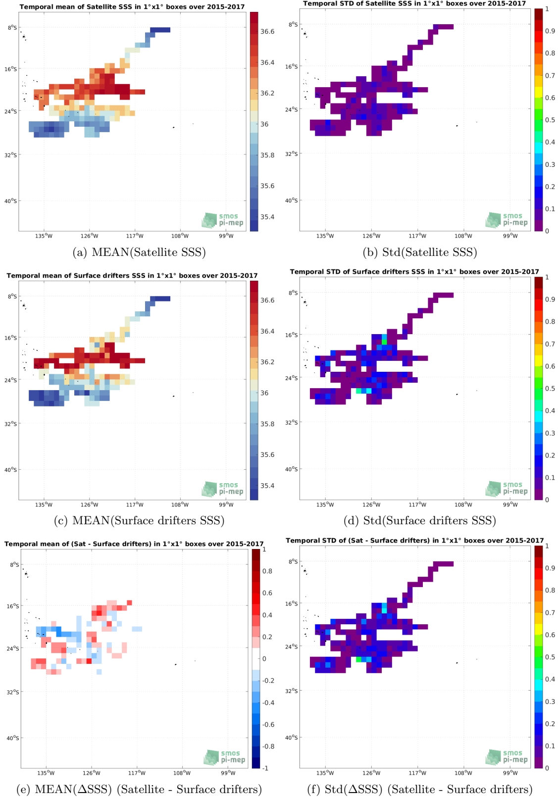
Figure 5: Temporal mean (left) and Std (right), of SSS from SMAP SSS L3 v4 - Monthly (RSS) (top), Surface drifters (middle), and of \Delta SSS (Satellite - Surface drifters). Only match-up pairs are used to generate these maps.
