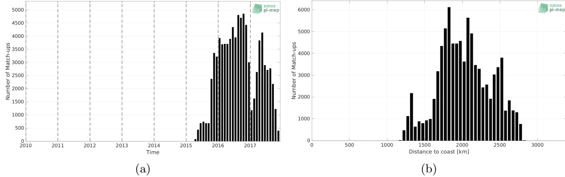
Figure 1: Number of match-ups between Surface drifters and SMAP SSS L3 v4 - Monthly (RSS) SSS as a function of time (a) and as function of the distance to coast (b) over the OTT zone Pi-MEP region and for the full satellite product period.
