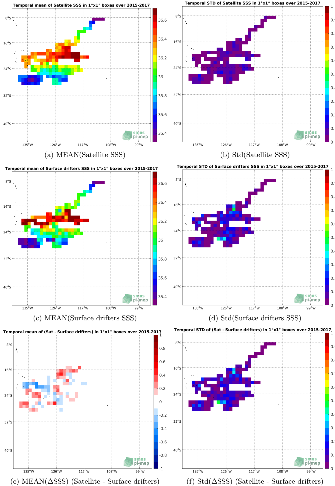
Figure 5: Temporal mean (left) and Std (right) of SSS from SMAP SSS L3 v4 - Monthly (RSS) (top), Surface drifters (middle), and of \Delta SSS (Satellite - Surface drifters). Only match-up pairs are used to generate these maps.
