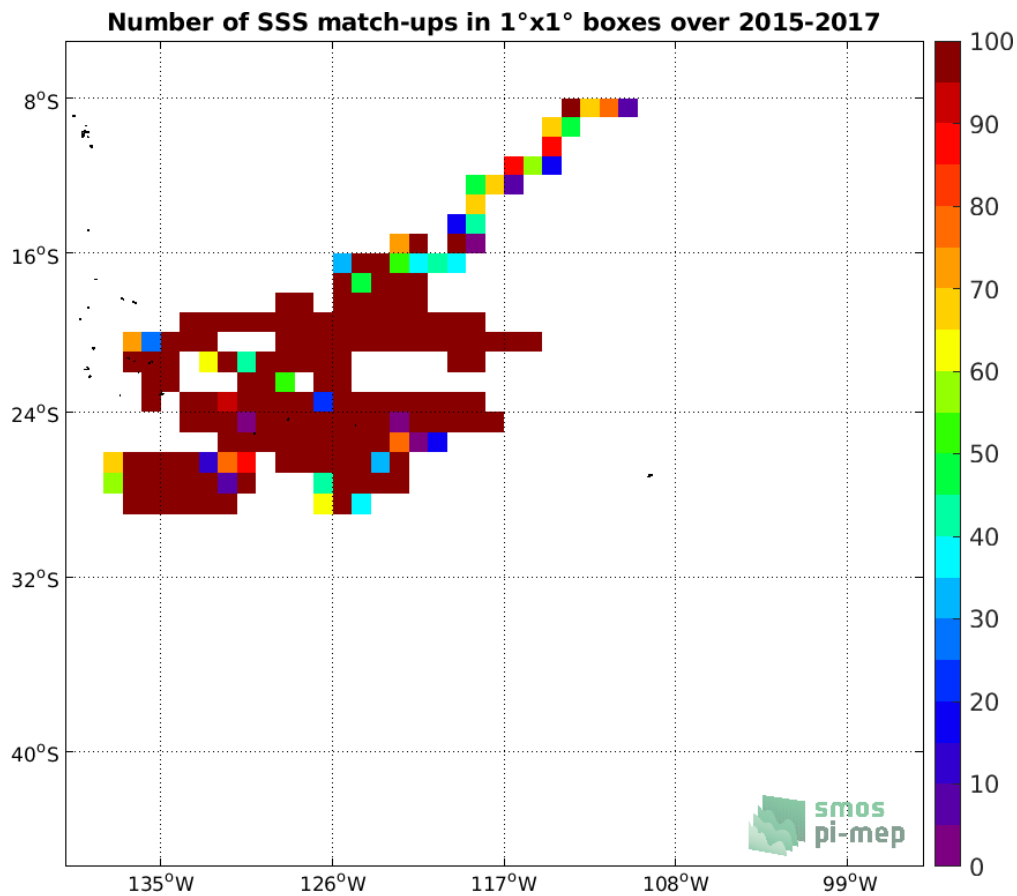
Figure 3: Number of SSS match-ups between Surface drifters SSS and the SMAP SSS L3 v4 - Monthly (RSS) SSS product for the OTT zone Pi-MEP region over 1°x1° boxes and for the full satellite product period.
