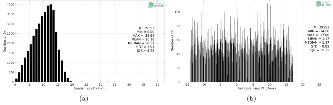
Figure 5: Histograms of the spatial (a) and temporal (b) lags between the location/time of the Argo measurement and the date of the corresponding SMAP SSS L3 v4 - Monthly (RSS) SSS pixel.
