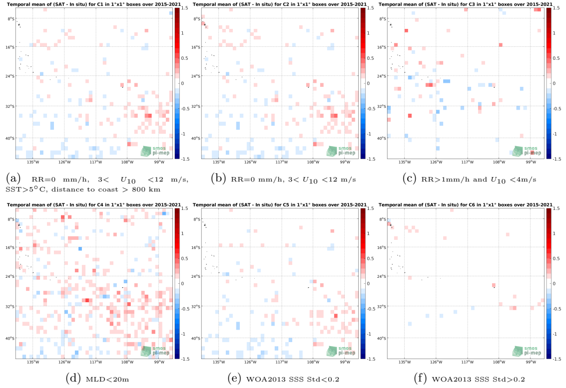
Figure 12: Temporal mean gridded over spatial boxes of size 1^\circ \times 1^\circ of \Delta SSS (SMAP SSS L3 v4 - Monthly (RSS) - Argo) for 6 different subdatasets corresponding to:RR=0 mm/h, 3 < U_{10} < 12 m/s, SST >5^\circ\text{C} , distance to coast > 800 km (a), RR=0 mm/h, 3 < U_{10} < 12 m/s (b), RR >1 mm/h and U_{10} < 4 m/s (c),MLD <20 m (d),WOA2013 SSS Std <0.2 (e),WOA2013 SSS Std >0.2 (f).
