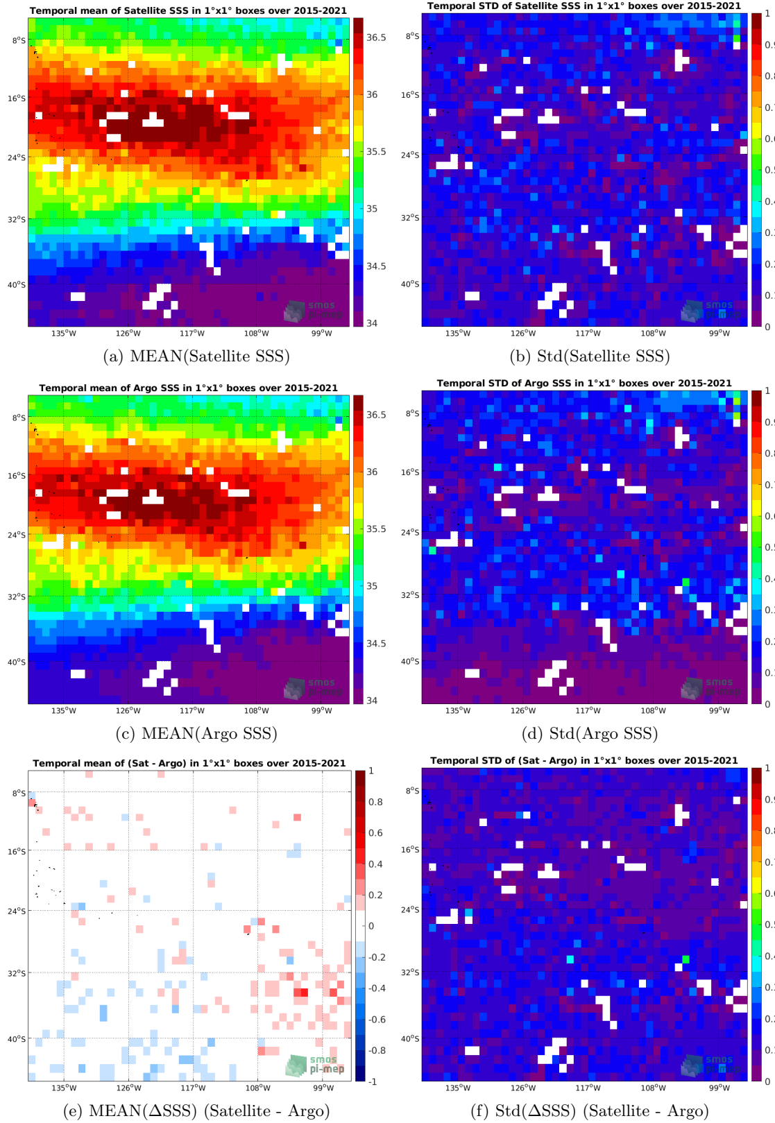
Figure 6: Temporal mean (left) and Std (right) of SSS from SMAP SSS L3 v4 - Monthly (RSS) (top), Argo (middle), and of \Delta SSS (Satellite - Argo). Only match-up pairs are used to generate these maps.
