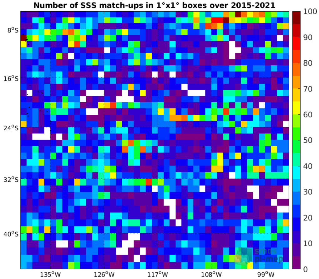
Figure 4: Number of SSS match-ups between Argo SSS and the SMAP SSS L3 v4 - Monthly (RSS) SSS product for the OTT zone Pi-MEP region over 1°x1° boxes and for the full satellite product period.
