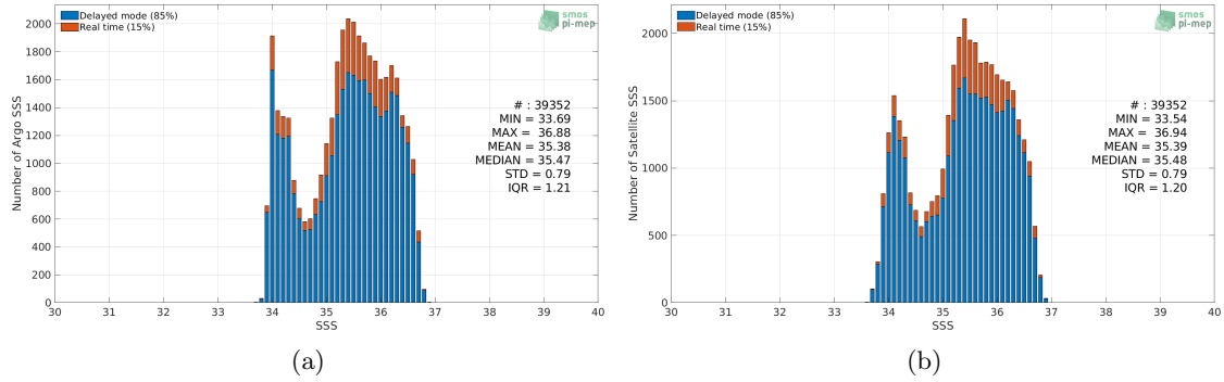
Figure 2: Histograms of SSS from Argo (a) and SMAP SSS L3 v4 - Monthly (RSS) (b) considering all match-up pairs per bins of 0.1 over the OTT zone Pi-MEP region and for the full satellite product period.
