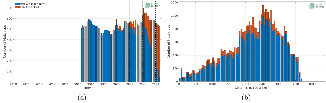
Figure 1: Number of match-ups between Argo and SMAP SSS L3 v4 - Monthly (RSS) SSS as a function of time (a) and as function of the distance to coast (b) over the OTT zone Pi-MEP region and for the full satellite product period.
