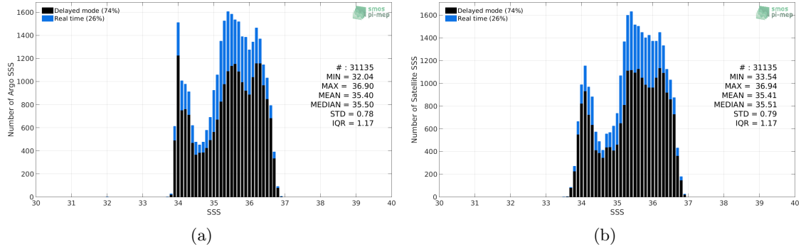
Figure 2: Histograms of SSS from Argo (a) and SMAP-L3-RSS-V4-MONTHLY (b) considering all match-up pairs per bins of 0.1 over the OTT zone Pi-MEP region and for the full satellite product period.
