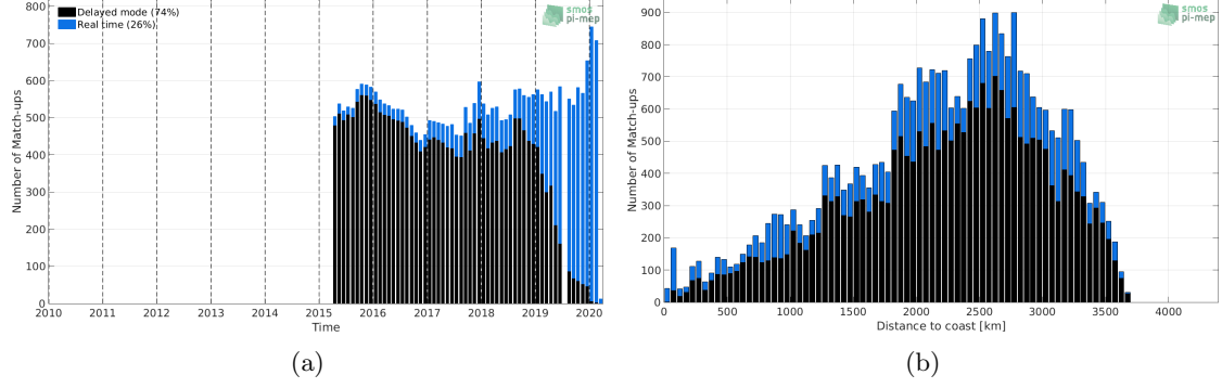
Figure 1: Number of match-ups between Argo and SMAP-L3-RSS-V4-MONTHLY SSS as a function of time (a) and as function of the distance to coast (b) over the OTT zone Pi-MEP region and for the full satellite product period.
