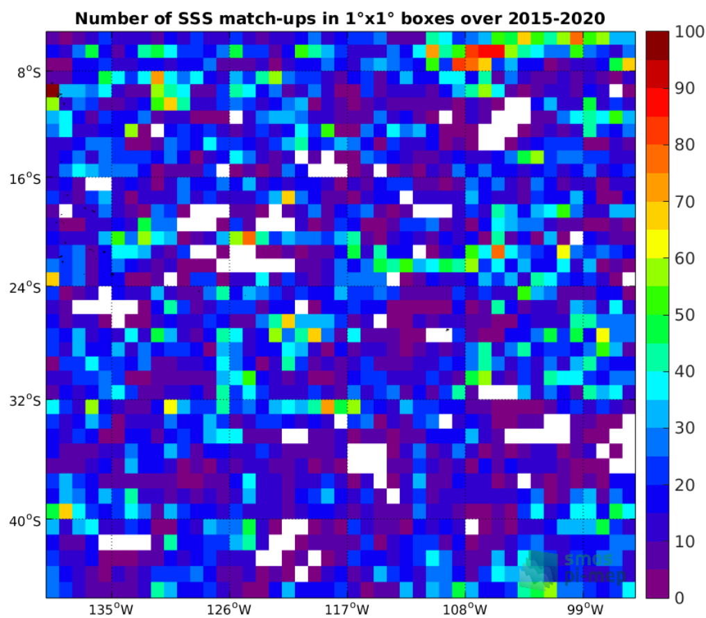
Figure 4: Number of SSS match-ups between Argo SSS and the SMAP-L3-RSS-V4-MONTHLY SSS product for the OTT zone Pi-MEP region over 1°x1° boxes and for the full satellite product period.
