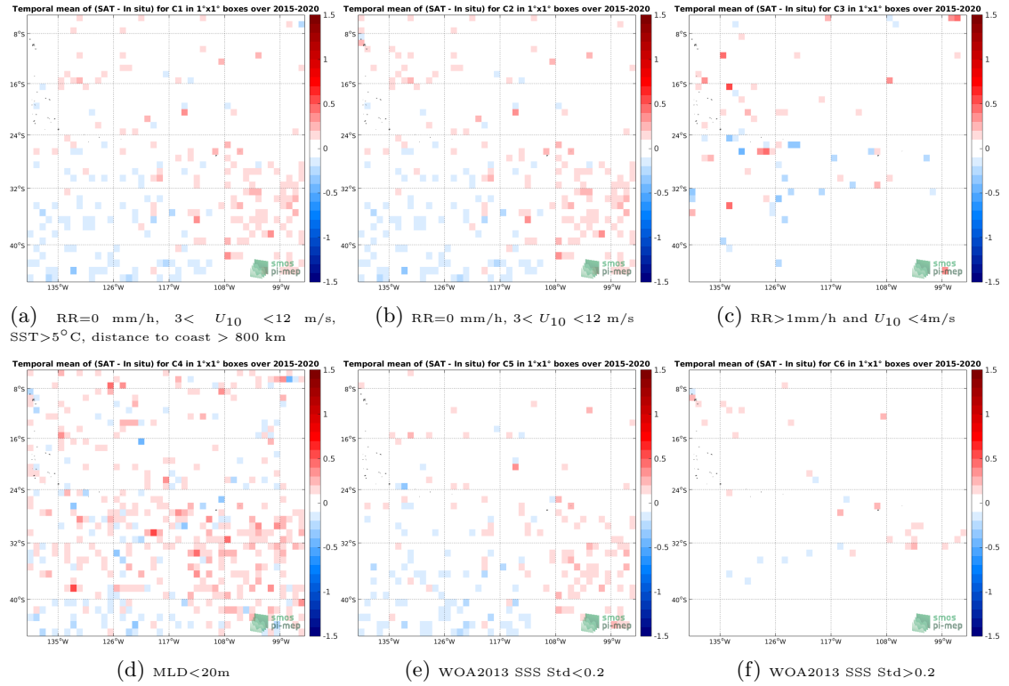
Figure 12: Temporal mean gridded over spatial boxes of size 1^\circ \times 1^\circ of \Delta SSS (SMAP-L3-RSS-V4-MONTHLY - Argo) for 6 different subdatasets corresponding to:RR=0 mm/h, 3 < U_{10} < 12 m/s, SST>5°C, distance to coast > 800 km (a), RR=0 mm/h, 3 < U_{10} < 12 m/s (b), RR>1mm/h and U_{10} < 4 m/s (c),MLD<20m (d),WOA2013 SSS Std<0.2 (e),WOA2013 SSS Std>0.2 (f).
