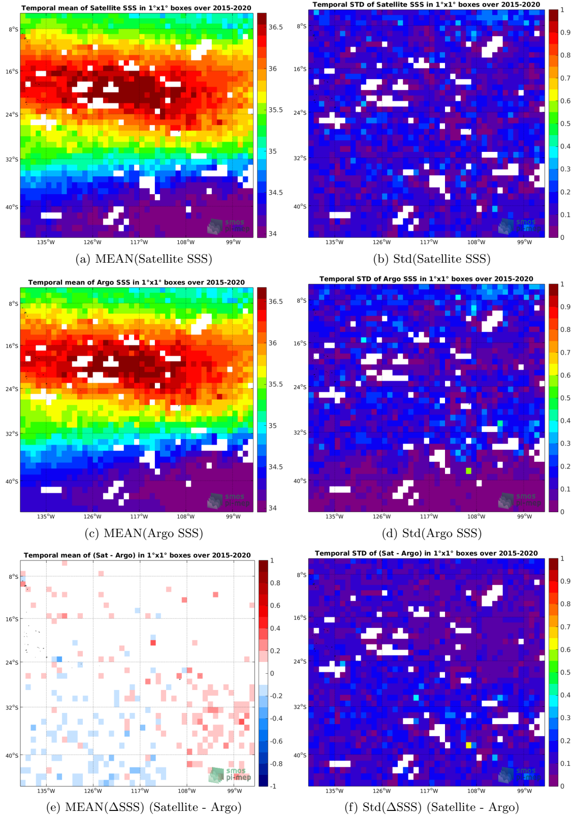
Figure 6: Temporal mean (left) and Std (right) of SSS from SMAP-L3-RSS-V4-MONTHLY (top), Argo (middle), and of \Delta SSS (Satellite - Argo). Only match-up pairs are used to generate these maps.
