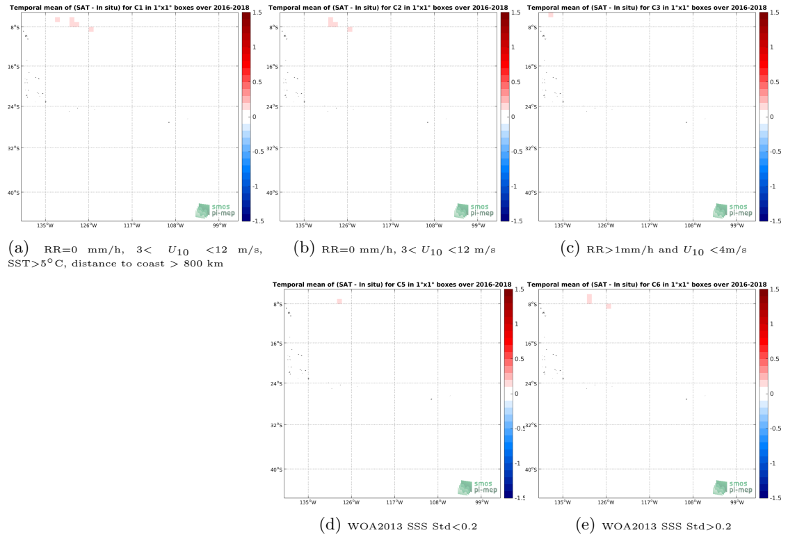
Figure 12: Temporal mean gridded over spatial boxes of size 1^\circ \times 1^\circ of \Delta SSS (SMAP-L3-RSS-V3-8DAY-RUNNING-70KM - TSG-SAMOS) for 5 different subdatasets corresponding to:RR=0 mm/h, 3 < U_{10} < 12 m/s, SST > 5^\circ\text{C} , distance to coast > 800 km (a), RR=0 mm/h, 3 < U_{10} < 12 m/s (b), RR > 1 mm/h and U_{10} < 4 m/s (c), WOA2013 SSS Std < 0.2 (d), WOA2013 SSS Std > 0.2 (e).
